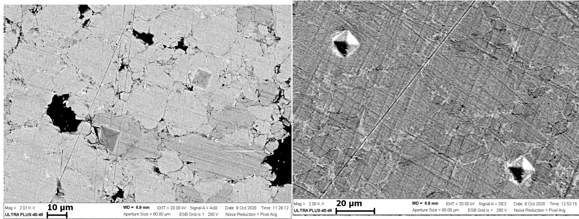
Figure S2. Microhardness prints in the samples sintered at 800 °C (a) and 1000 °C (b).
