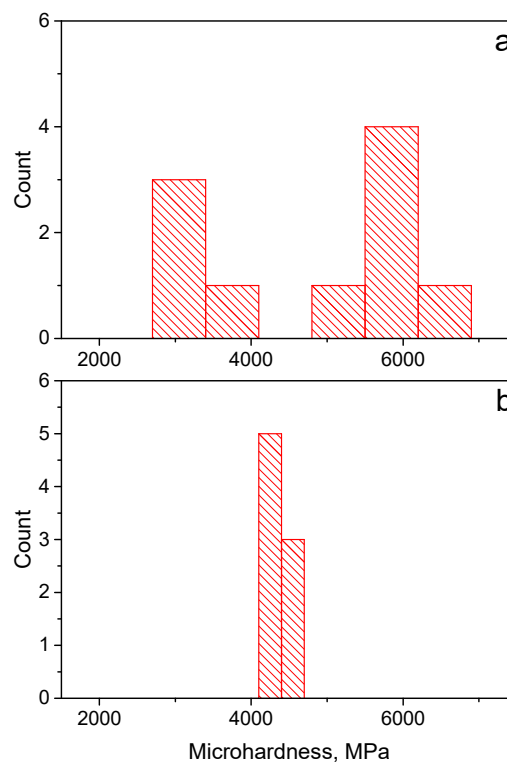
Figure S1. Distributions of microhardness measured in different randomly chosen points of the SPS-consolidated samples: SPS at 800 °C (a) and SPS at 1000 °C (b).
