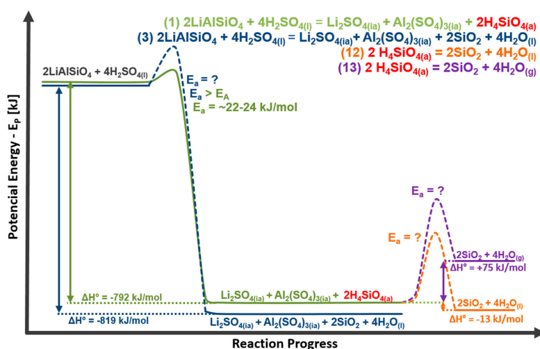
Figure 15. Potential energy diagram of \text{LiAlSiO}_4 phase leaching with the focus on the silicon phases.
