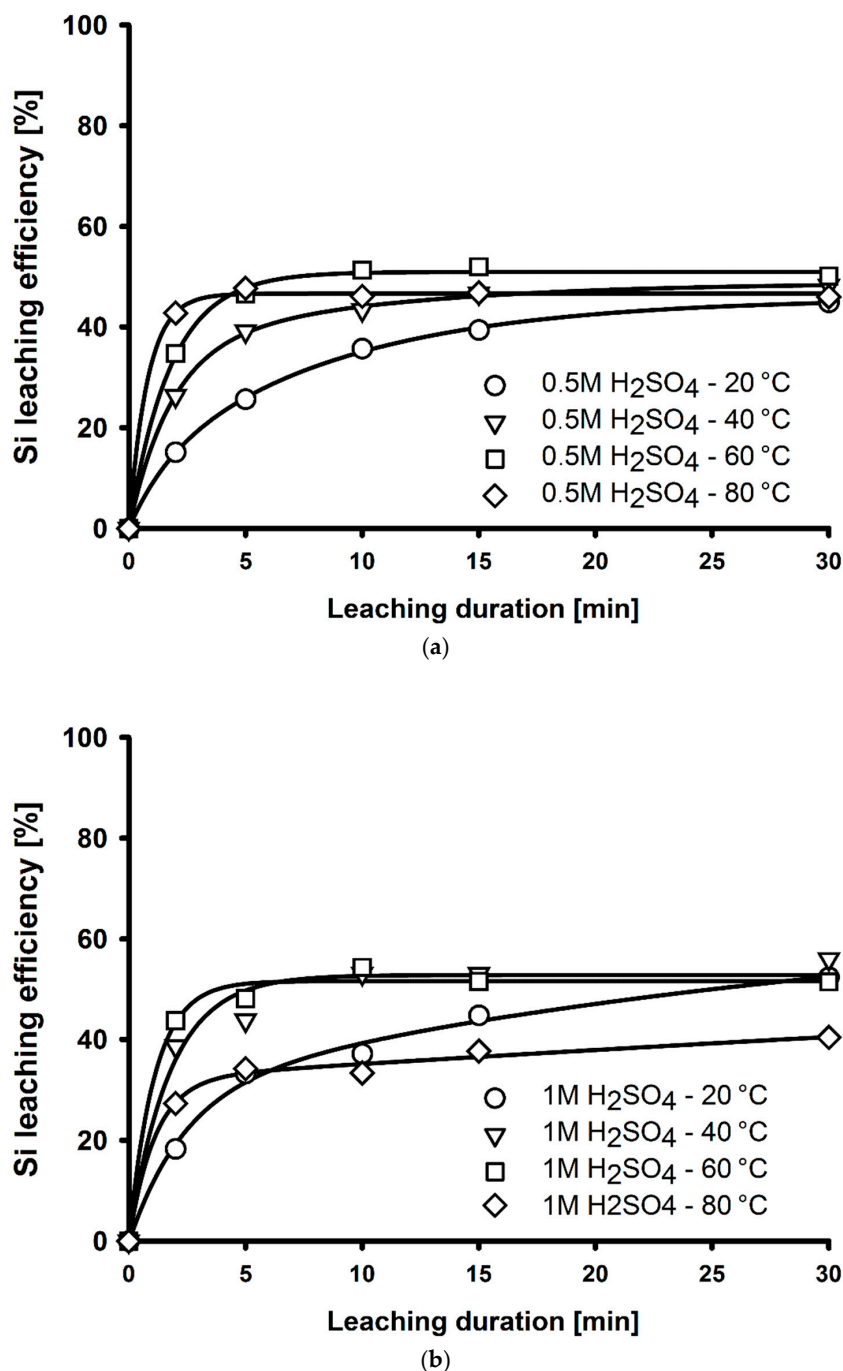
Figure 9. Silicon leaching efficiency at 20–80 °C in 0.5 M (a) and 1 M (b) H_2SO_4 .
