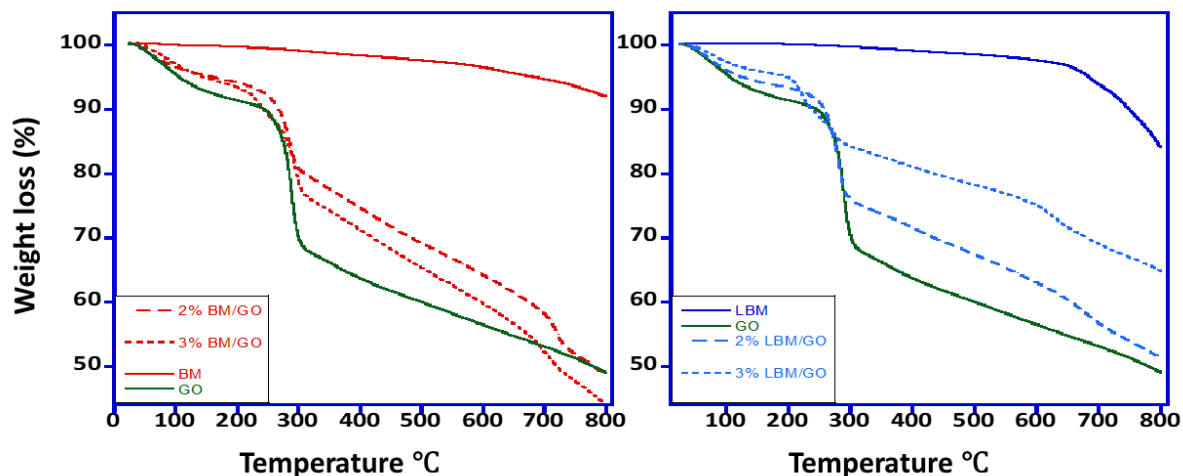
Figure S1: Comparative thermal degradation patterns of (a) BM, LM, GO, 2% BM/GO 3% BM/GO, 2% LBM/GO, and 3% BM/GO
