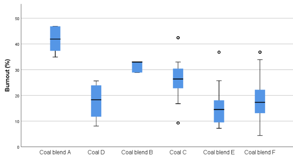
Figure 15. Range of coal burnout for each of the coals/coal blends used during observed blast furnace production (○ = high/low potential outliers).
