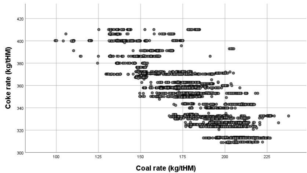
Figure 7. Scatter plot of the relationship between the injectant coal and the coke rate during blast furnace production.
