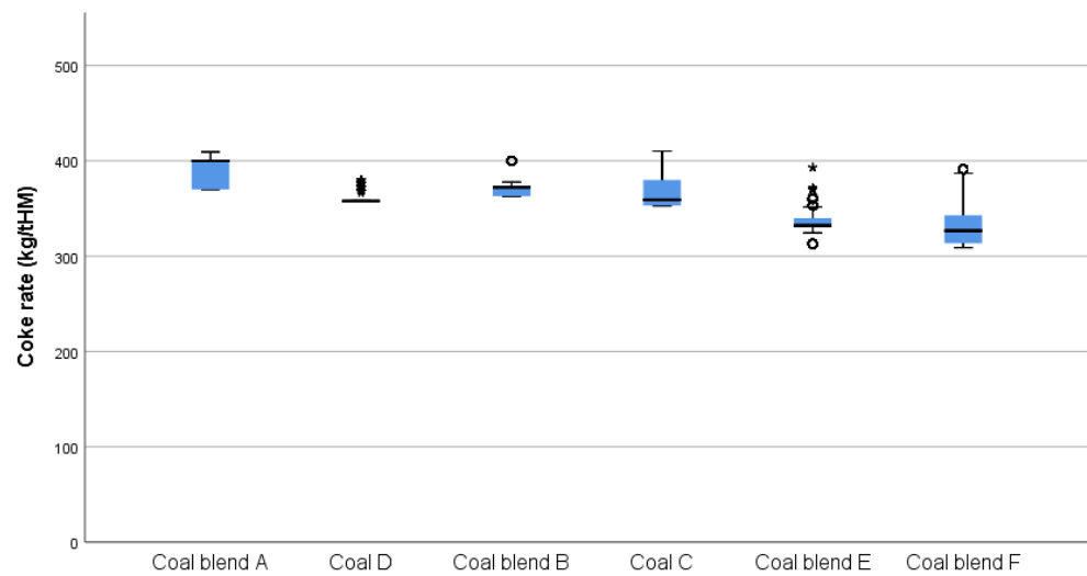
Figure 13. Box plots of the range of coke addition rates for the time periods corresponding to the addition of different coals/coal blends during blast furnace production ( \circ = high/low potential outliers and * = high/low extreme values).
