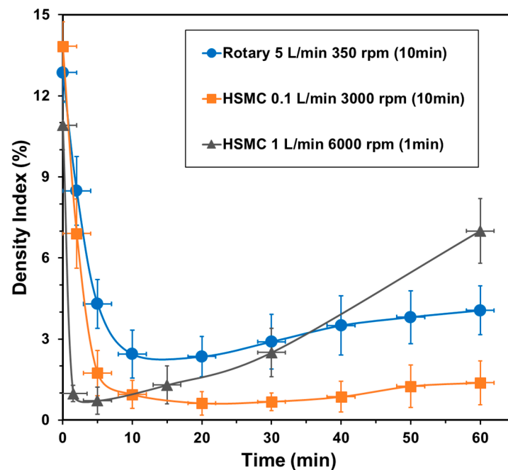
Figure 5. Comparison by Density Index evaluation of the HSMC degassing performance with conventional rotary degassing. Data points replotted from results in previous studies [24,32].
