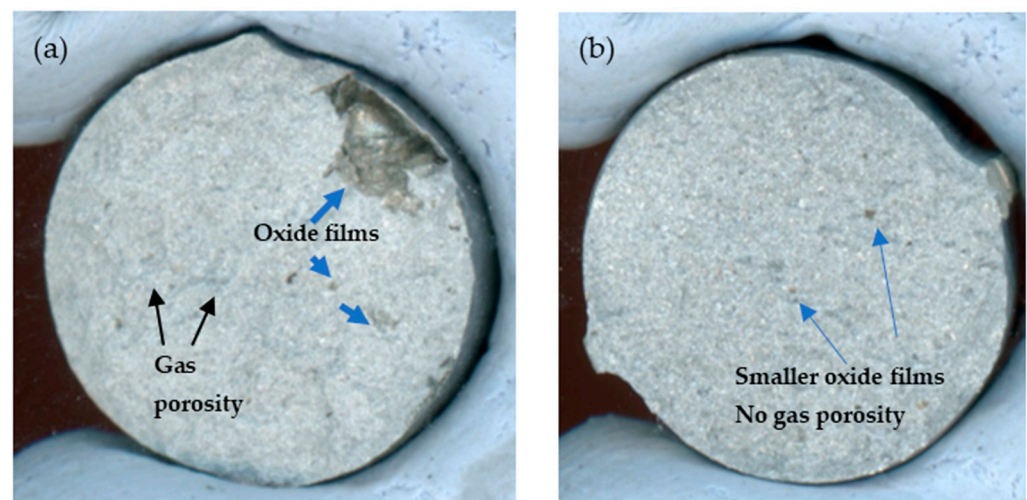
Figure 8. Fracture surfaces of postmortem tensile bars that were cast after (a) conventional rotary degassing and (b) HSMC degassing. Representative samples are from a previous study [24].
