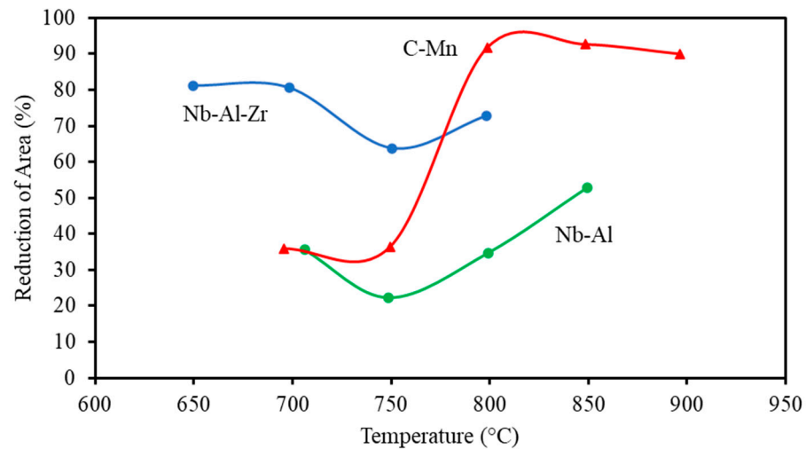
Figure 20. Hot ductility curves for plain C-Mn, C-Mn-Nb-Al, and C-Mn-Nb-Al-Zr steels. Tensile samples were solution-treated at 1330 °C, then cooled to the test temperature at 60 °C/min and strained at a rate of 3 \times 10^{-3} \text{ s}^{-1} [108], with the permission from Taylor & Francis, 2023.
