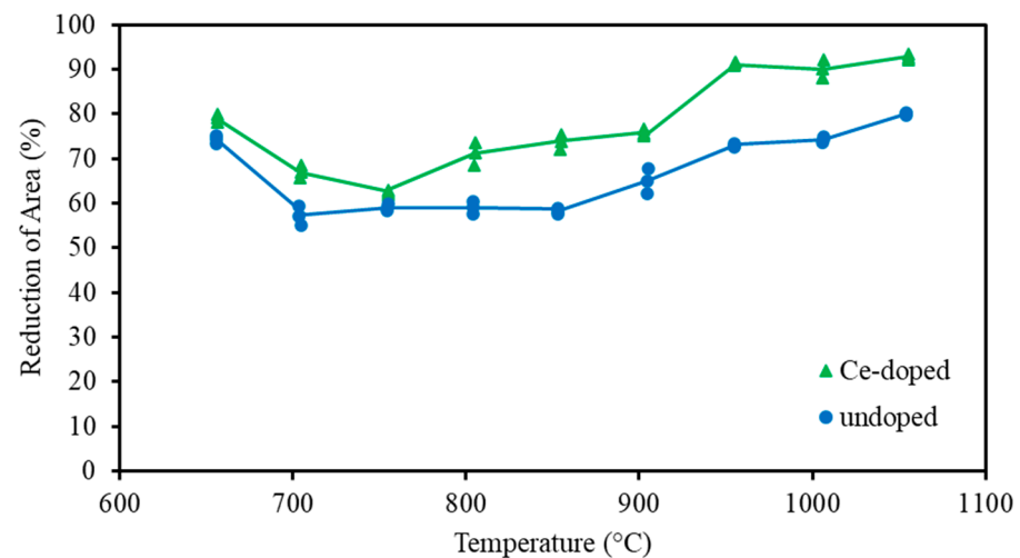
Figure 15. The hot ductility curves of reactor pressure-vessel steel that is both un-doped and doped with 0.07% Ce. The base composition of the steel was 0.18% C, 0.22% Si, 1.45% Mn, 0.75% Ni, and 0.5% Mo [89]. Adapted from [89], with permission from Elsevier, 2023.
