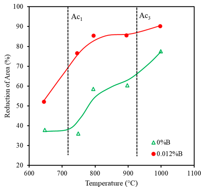
Figure 10. Influence of the addition of B (0.012%) on the hot ductility curve of low-carbon advanced high-strength steels (AHSS). The base composition of the steel was 0.06% C, 0.35% Mn, 0.3% Si, 2.2% Ni, 1.2% Cr, 0.5% Cu, 0.2% V, and 0.006% N, and was Ti-free [58]. Adapted from [58], with permission from Elsevier, 2023.
