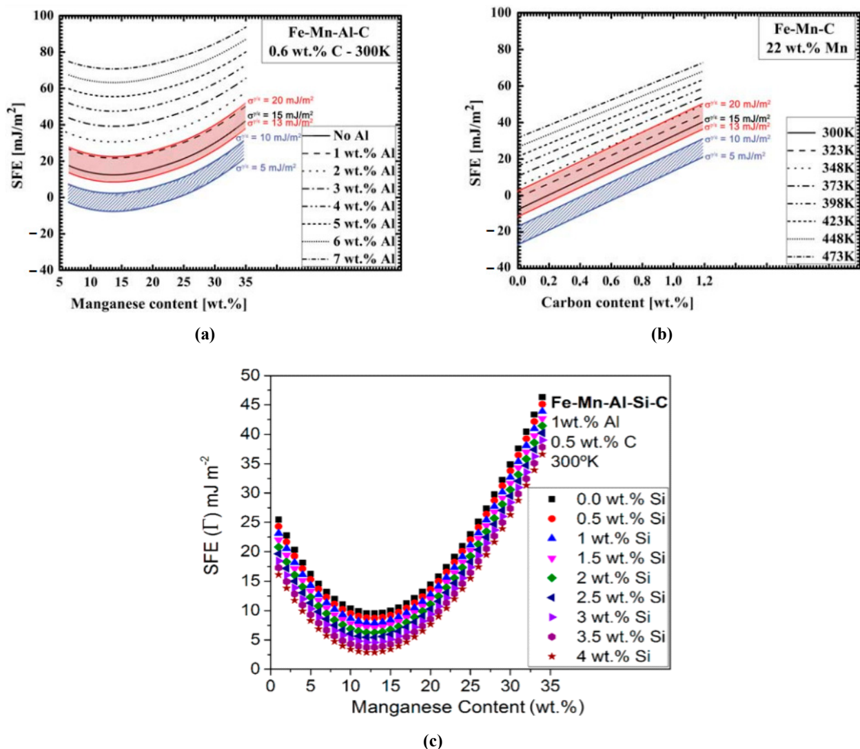
Figure 14. Composition-dependent SFE maps. (a) The influence of Mn and Al contents on SFE in a steel with 0.6% C [71]. Adapted from [71], with permission from Springer, 2023. (b) The influence of C content on the SFE in a steel with 22% Mn [71]. (c) The influence of Mn and Si on the SFE in a 0.5% C steel with 1% Al [64]. Adapted from [64], with permission from ASME Publications, 2023.
