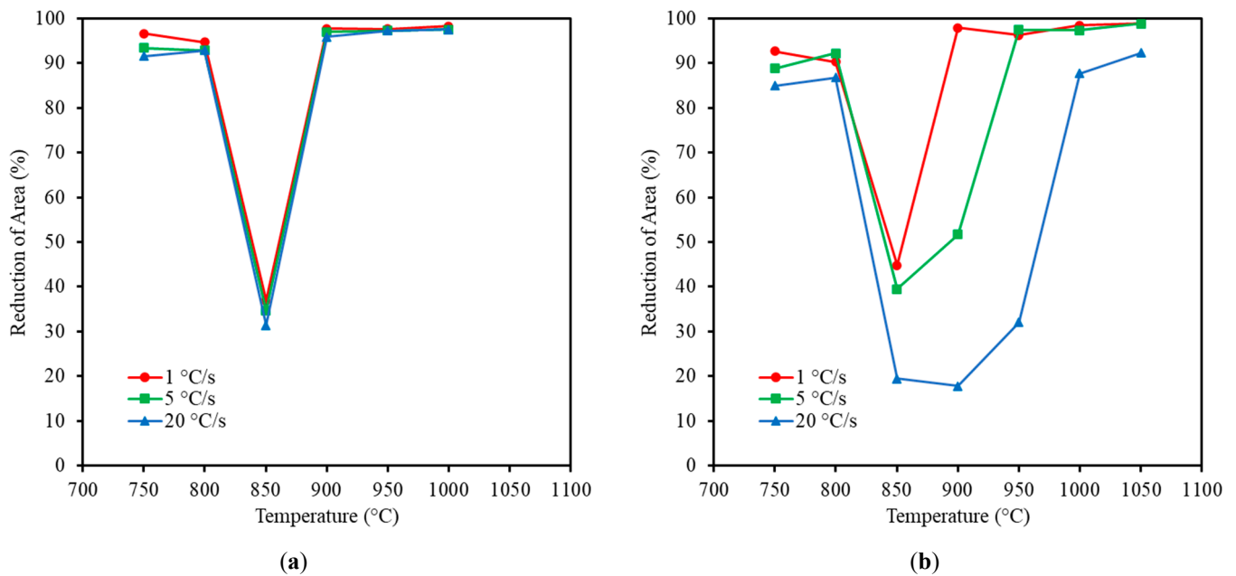
Figure 9. Hot ductility curves at various cooling rates for: (a) B-free steel and (b) B-containing steel [45]. Adapted from [31], with permission from Springer, 2023.
