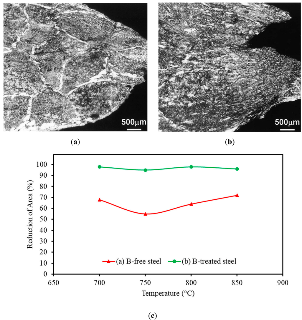
Figure 6. The change in ferrite distribution from the boundaries to the matrix by adding 0.002% B, in samples tested at 750 °C. (a) No B, ferrite at boundaries; (b) with 0.002% B addition, ferrite was distributed at the boundaries and within the matrix; (c) hot ductility curves for the two steels [30]. Adapted from [30], with permission from Elsevier, 2023.
