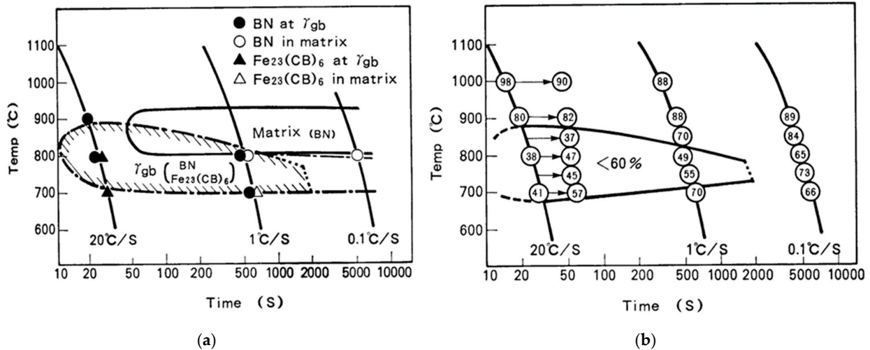
Figure 11. (a) PTT (precipitation–temperature–time) diagram for BN precipitation, both in the matrix and at grain boundaries. (b) Temperature–time–ductility diagram for boron-treated steels, with the cooling rate curves for 3 different cooling rates, 20 °C/s, 1 °C/s, and 0.1 °C/s. The temperature range that yields lower ductility widens as the cooling rate increases, ductility occurring for all test temperatures at 0.1 °C/s with > 60%RA, decreases to 50%RA between 700 °C to 800 °C for the cooling rate of 1 °C/s, decreases further to 40%RA for the highest cooling rate 20 °C/s, and spans the widest temperature range of 670 °C to 870 °C. The numbers in circles are the RA values [44].
