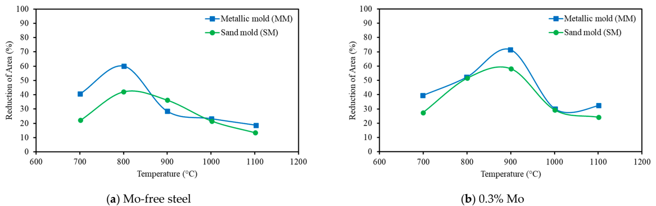
Figure 4. Hot ductility curves of the as-cast TWIP steel, having a base composition of 0.5% C, 21% Mn, 1.3% Si, 1.5% Al, and 0.012% N: (a) with no Mo present in the steel; (b) a 0.3% Mo addition. Tensile specimens were machined from sand molds or ingot castings, so as to give two cooling rates, a slow cooling rate with the sand molds and a fast cooling rate with the metallic molds. The 0.3% Mo addition can be seen to improve ductility in the intermediary temperature range of 800 to 950 °C, independent of the cooling conditions [13]. Adapted from [13], with permission from Elsevier, 2023.
