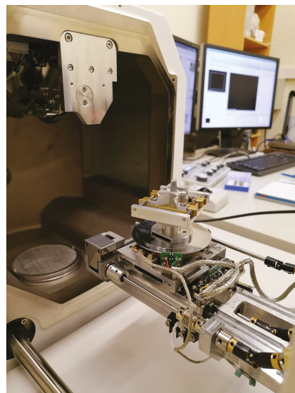
Figure 3. Specimen setup for SEM analysis.
