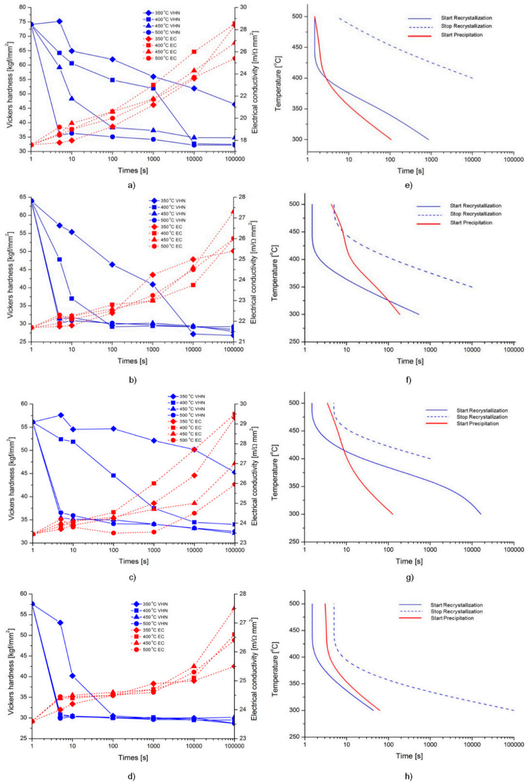
Figure S1. (a) Vickers hardness and electrical conductivity (EC) for the different materials material with the true strain of \epsilon = 3.0 during isothermal back annealing at 350 °C, 400 °C, 450 °C and 500 °C for different times (a–d) and TTT-diagrams (e–g) for C2-0 (a,e); C2-1 (b,f); C2-2 (c,g) and C2-3 (d,h).
