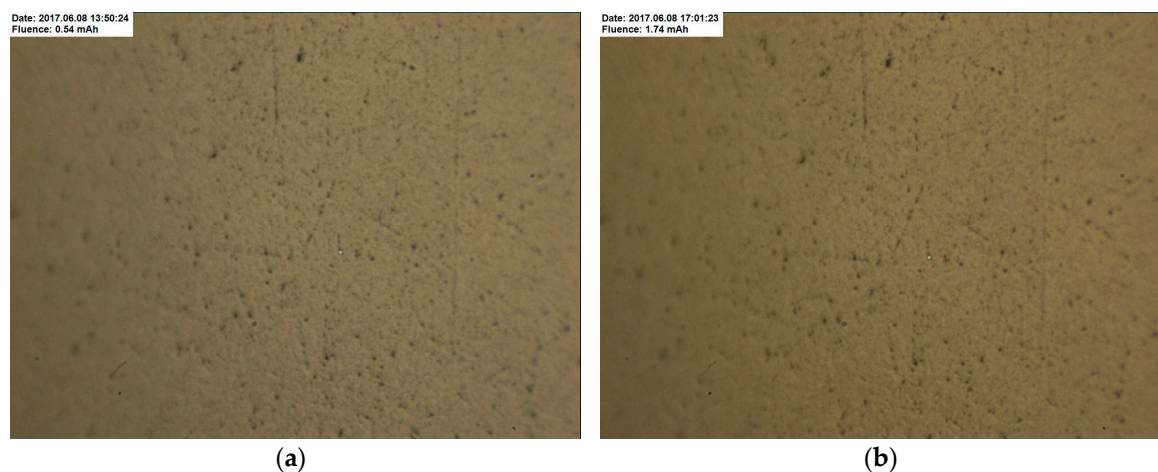
Figure 22. Images of the surface of Sample 5 during irradiation by a 2-MeV proton beam with varying integrals of the current: (a) 0.54, (b) 1.74 mA·h. The frame size is 9 mm horizontally and 4 mm vertically.
