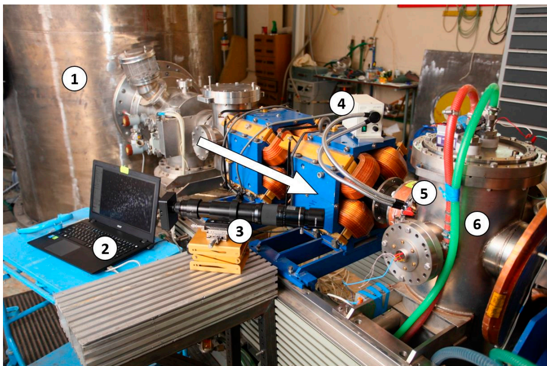
Figure 1. Experimental apparatus: ①, tandem accelerator with vacuum insulation; ②, computer; ③, remote microscope with a charge-coupled device camera; ④, booster-light; ⑤, fused quartz window; and ⑥, diagnostic vacuum chamber. The arrow schematically shows the direction of 2-MeV proton beam propagation.
