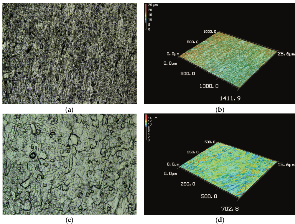
Figure 7. Laser microscope images of the tantalum surface and the results of their processing: (a,b), non-irradiated; (c,d), irradiated. The frame size is (a,b), 1411.9 \times 1000 \mu\text{m}^2 ; (c,d), 702.8 \times 500 \mu\text{m}^2 ; the height is (b) 25.6 \mu\text{m} ; (d) 15.6 \mu\text{m} .
