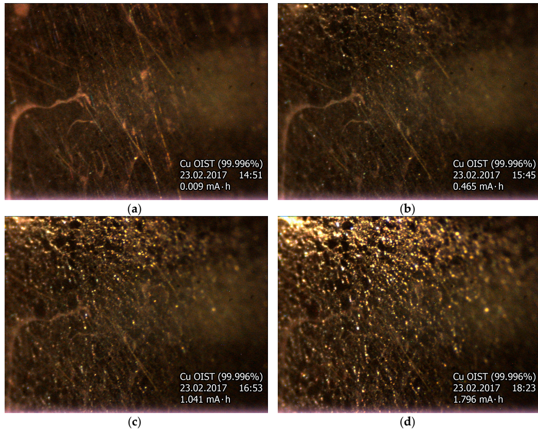
Figure 3. Images of the surface of 99.996% fine copper irradiation by a 2-MeV proton beam with varying integrals of the current: (a) 0.009; (b) 0.465; (c) 1.041; (d) 1.796 mA·h. The frame size is 9 mm horizontally and 4 mm vertically.
