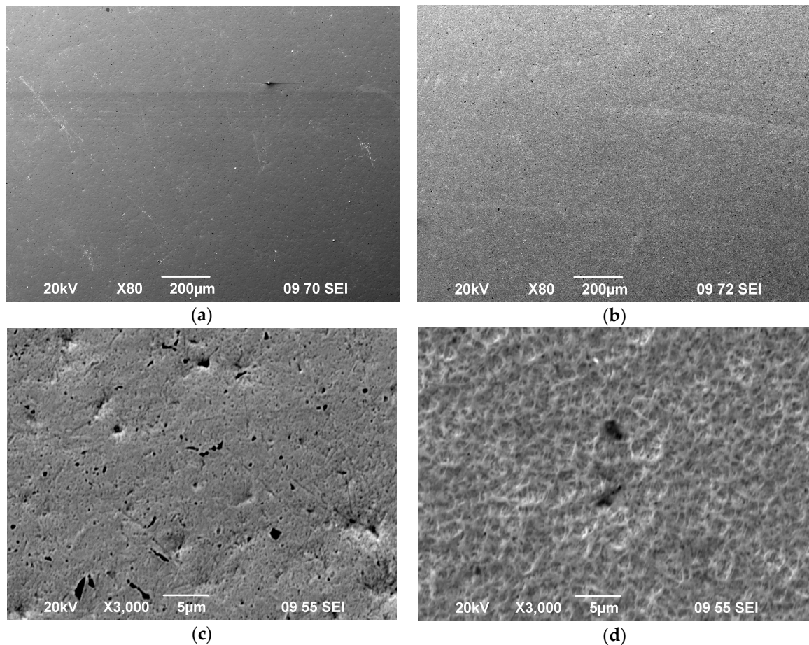
Figure 24. Images of the surface of Sample 6 taken on a Jeol JCM-5700 electron microscope before (a,c) and after irradiation to a fluence of 6.7 \times 10^{20} \text{ cm}^{-2} (b,d).
