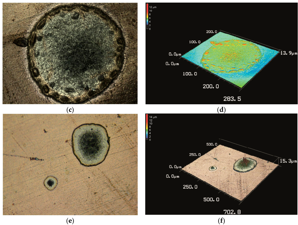
Figure 4. Laser microscope image of the M0 copper surface and the results of their processing: (a,b), non-irradiated; (c–f), irradiated. The frame size is (a,b), 1411.9 \times 1000 \mu\text{m}^2 ; (c,d), 283.5 \times 200 \mu\text{m}^2 ; (e,f), 702.8 \times 500 \mu\text{m}^2 ; the height is (b) 6.7 \mu\text{m} ; (d) 13.9 \mu\text{m} ; (f) 15.3 \mu\text{m} .
