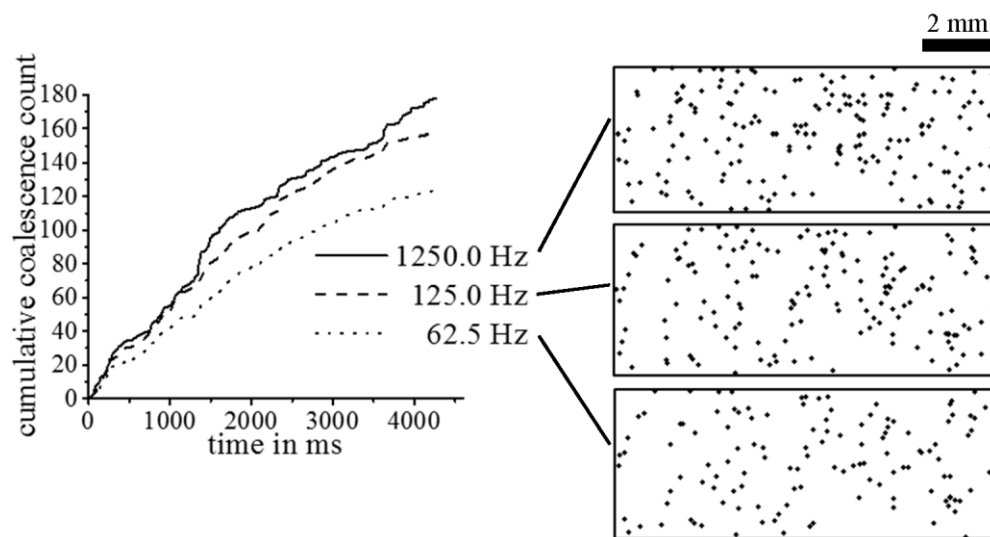
Figure 3. Cumulative coalescence count vs. time and coalescence maps of a uniaxially hot-compacted AlSi6Cu4 + 0.5 wt % TiH 2 sample detected with image acquisition rates of 1250 Hz (compact line), 125 Hz (dashed line), 62.5 Hz (dotted line) with corresponding coalescence maps.
