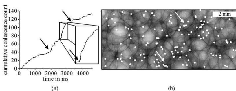
Figure 2. (a) Cumulative coalescence count vs. time with black arrows showing exemplary the starting point of three avalanches (one magnified as inset) and (b) coalescence map of a thixocast AlSi 6 Cu 4 + 0.5 wt % TiH 2 liquid foam. White arrows indicate examples for close spatial distances between film ruptures. Each point in both images represents one single coalescence. A video of the whole sequence can be found online in the Supplementary Materials (Video S1).
