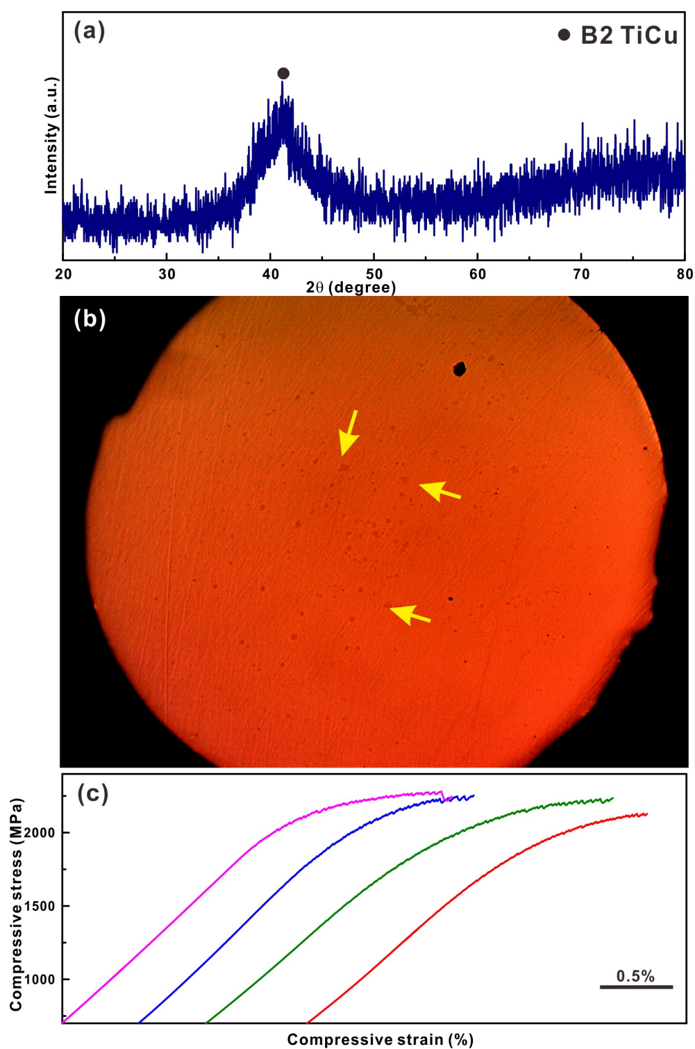
Figure S1. (a) XRD pattern, (b) OM image, and (c) room temperature engineering stress-strain curves of the as-cast T5 samples under compression.
