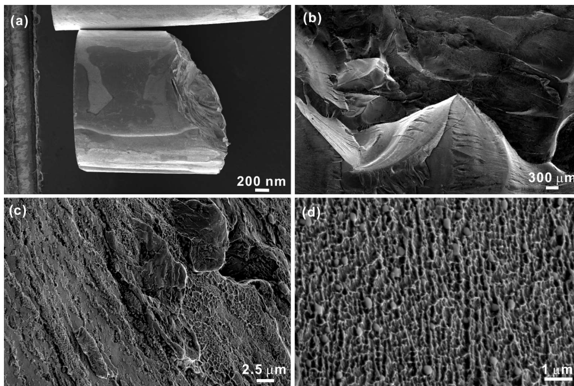
57 Figure S2. (a) the surface morphology and (b-d) the fracture morphology of the as-cast T5 samples under 58 compression. 59
