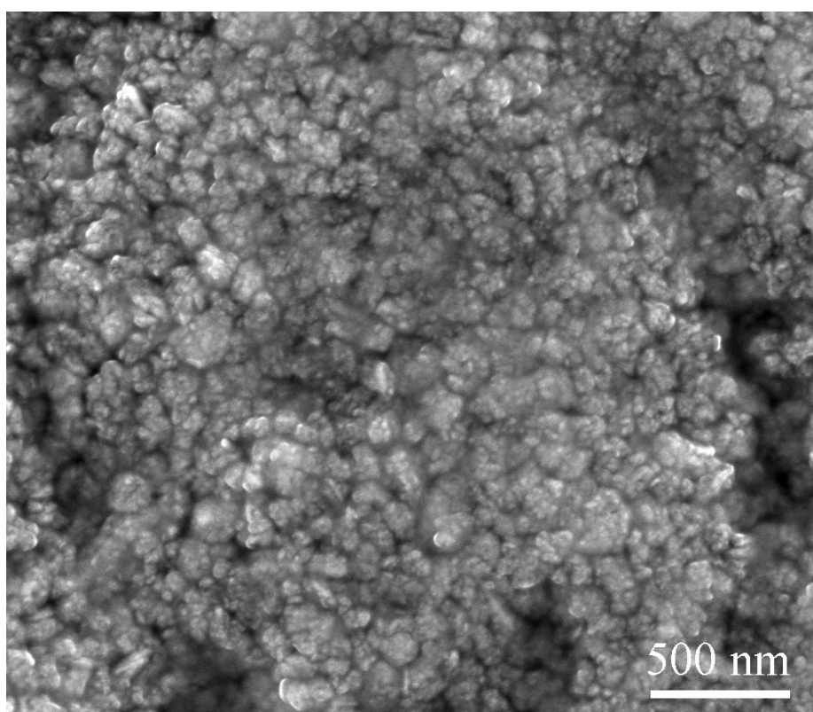
Figure S2. The SEM images of ball milled tungsten powder at 60 h with milling speed of 700 rpm and 8% PCA (process control agent). It shows two or more particle agglomerate together and form one large particle cluster.
