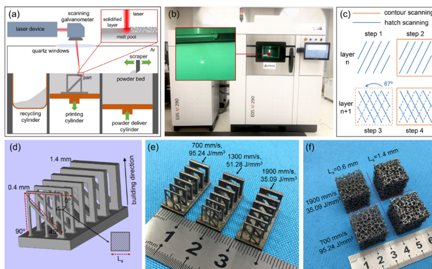
Figure 2. (a) Schematic of the laser powder bed fusion process; (b) the LPBF machine of EOS M290; (c) the selected scanning strategy; (d) the as-designed 3D model of solid struts; (e) the as-built Ti–6Al–4V solid struts; and (f) the as-built Ti–6Al–4V porous structures for the confirmatory experiment.
