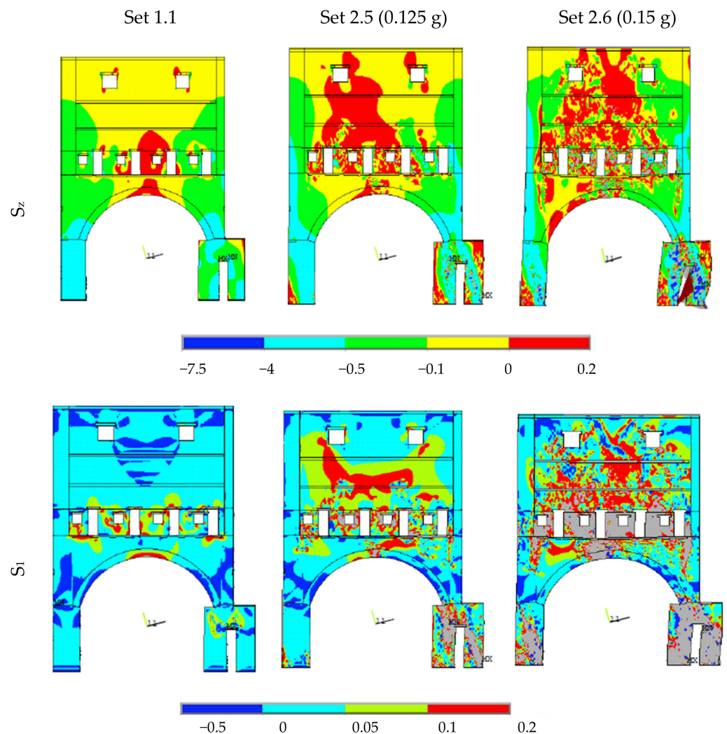
Figure 15. Stress state in [N/mm^2] at the end of different set of analysis.
