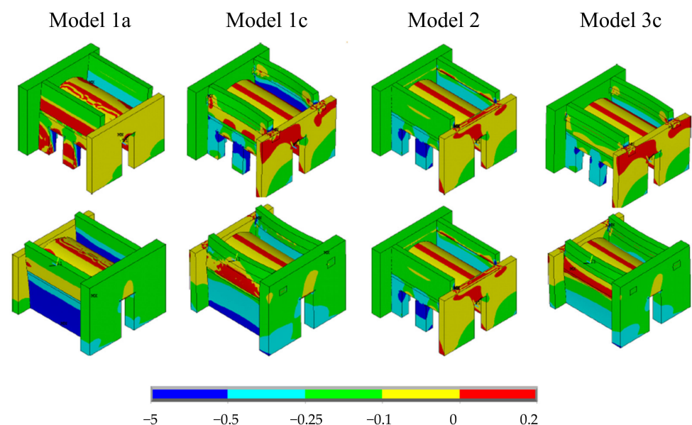
Figure 20. Vertical stresses in [\text{N}/\text{mm}^2] in the walls (Set 2.3 of Table 9).
