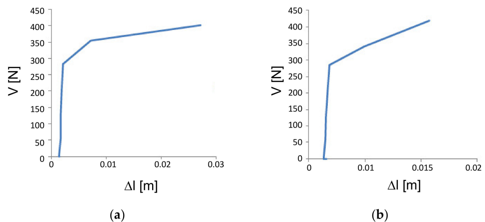
Figure 22. Relative displacement between pillars ( \Delta l ) vs. shear ( V ) obtained with the two hypotheses of interventions: (a) Sol (i); (b) Sol (ii).
