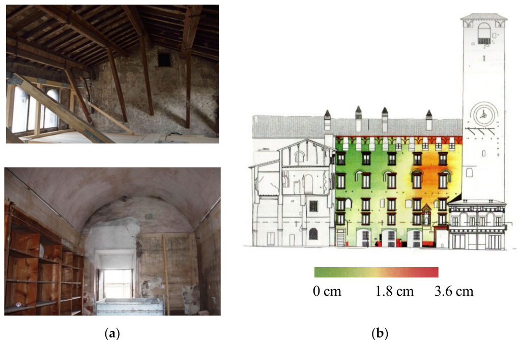
Figure 4. (a) Floors types (timber diaphragms and vaults); (b) out-of-plane deformations on the façade overlooking the Broletto square from laser scanner measurements made before and after the seismic event.
