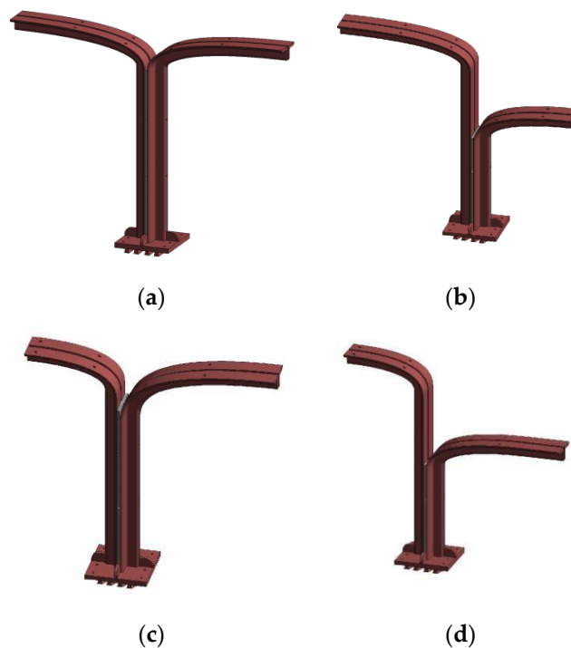
Figure 10. Parameterised units of different configurations. (a) Standard unit; (b) Unit with the same span but different heights; (c) Unit with the same height but different spans; (d) Unit with different heights and spans.
