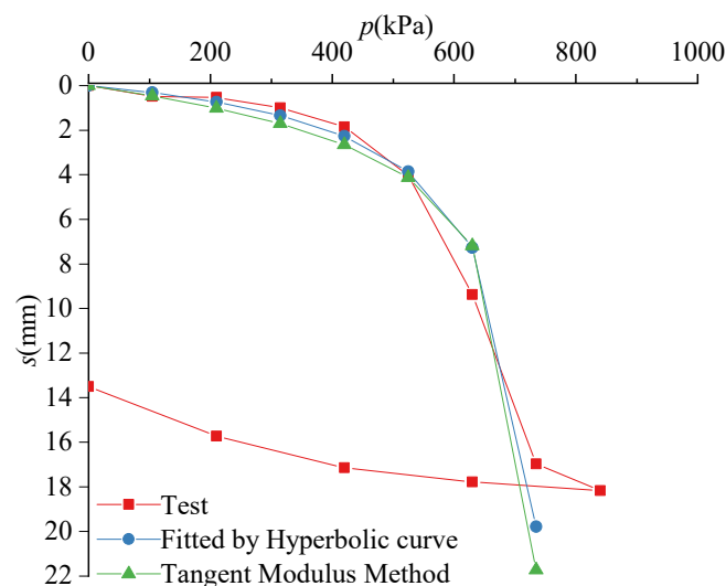
Figure 6. Comparison of p - s curve.
