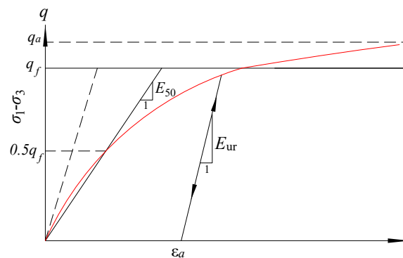
Figure 1. Unloading–reloading stress–strain curves.
