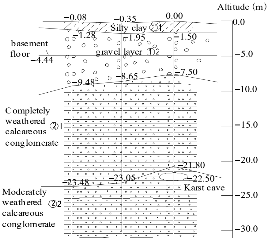
Figure 11. Typical geological profile of 15# building.
