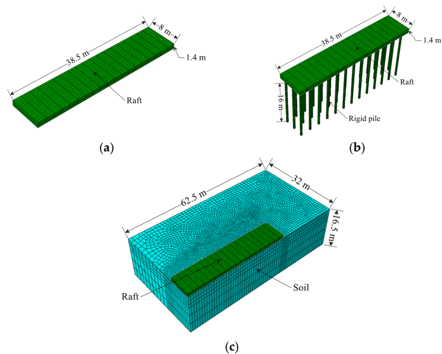
Figure 14. Finite element model of rigid pile composite foundation of Building 15: (a) raft; (b) raft and pile; and (c) FEM model.
