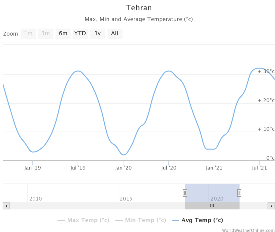
Figure 3. Weather temperatures throughout three years in Tehran [44].
