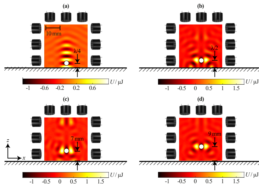
Figure 6. Force potential for (a) a standing wave with a minimum at z = \lambda/4 , and VTTs at (b) z = \lambda/2 , (c) z = 7 mm, and (d) z = 9 mm. The potentials are obtained for an acoustically reflective surface ( R = 1 ) at z = 0 .
