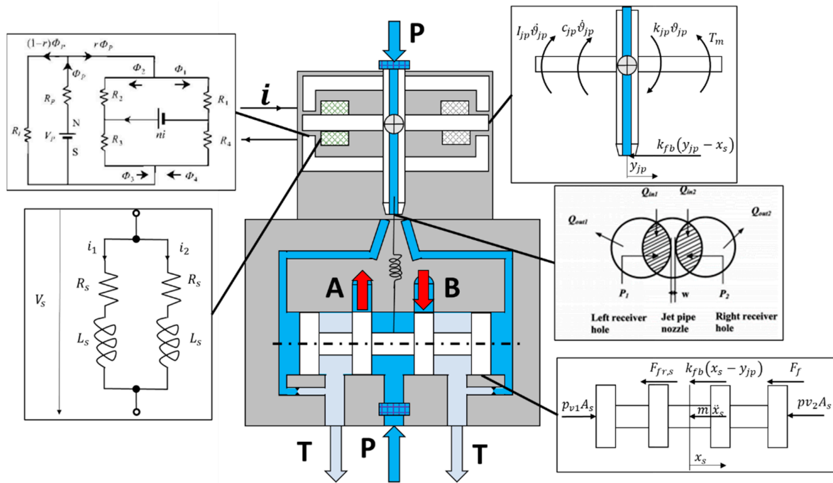
Figure 2. Schematics and modeling of a jet-pipe servovalve.
