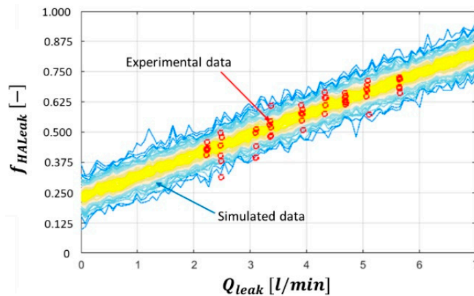
Figure 7. Feature behavior for increasing internal leakage.
