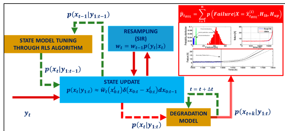
Figure 9. Flowchart of the prognostic algorithm.
