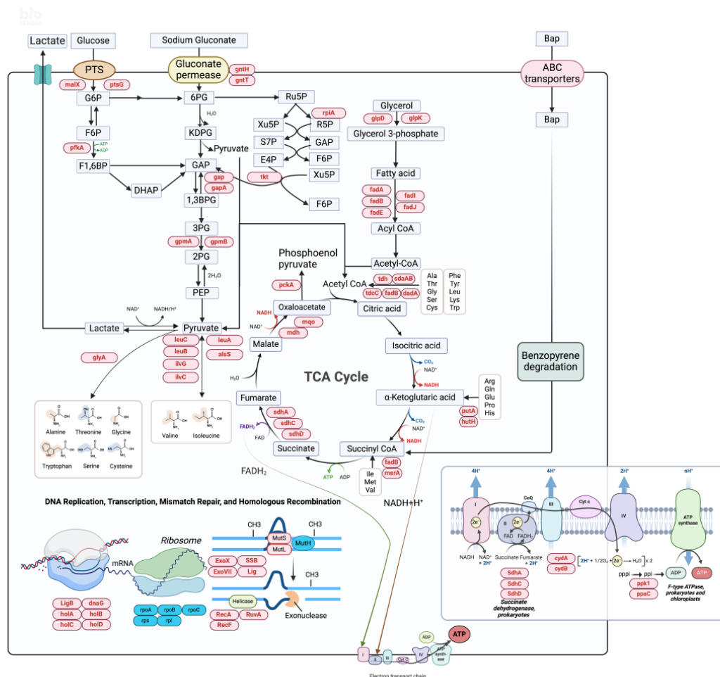
Figure 7. DEGs analysis of MSC14 stimulated by sodium gluconate. The genes highlighted within the red boxes in the figure indicate upregulated genes, while those within the blue boxes represent downregulated genes, the blue box represents substances related to metabolism, The brown box represents amino acids, Enlarged illustration of the Electron transport chain in the lower-right quadrant of the image. Figure 7 was created with biorender.com.
