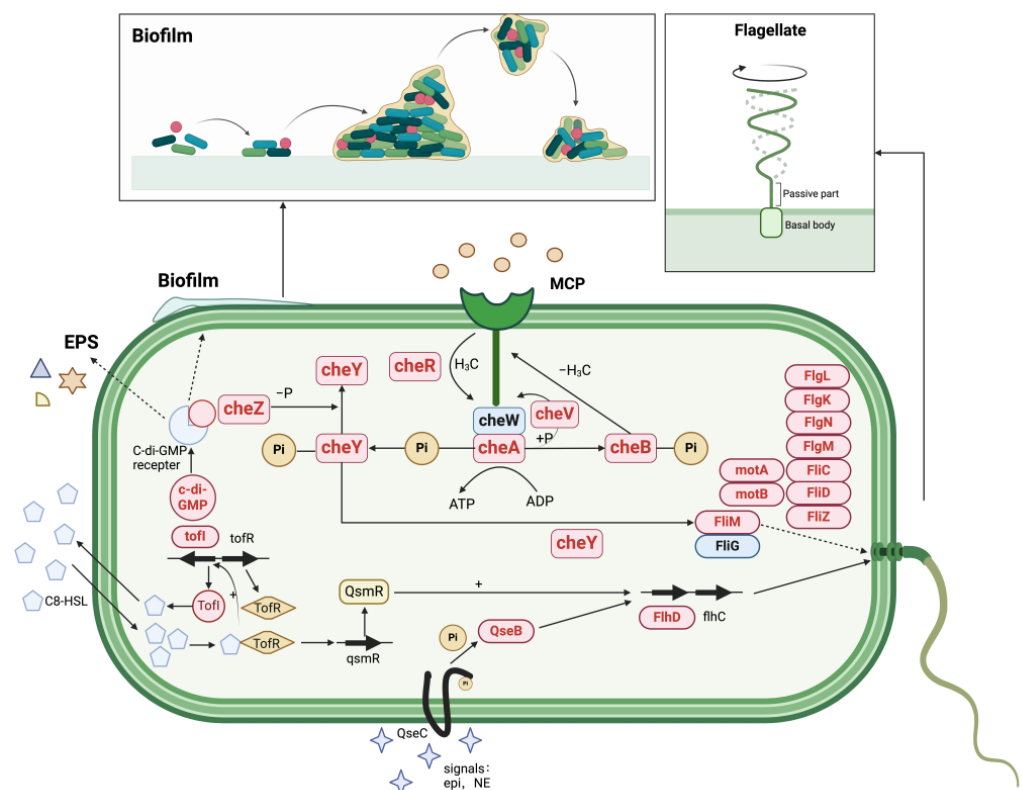
Figure 8. Regulation of MSC14 QS system stimulated by sodium gluconate. The genes highlighted within the red boxes in the figure indicate upregulated genes, while those within the blue boxes represent downregulated genes.
