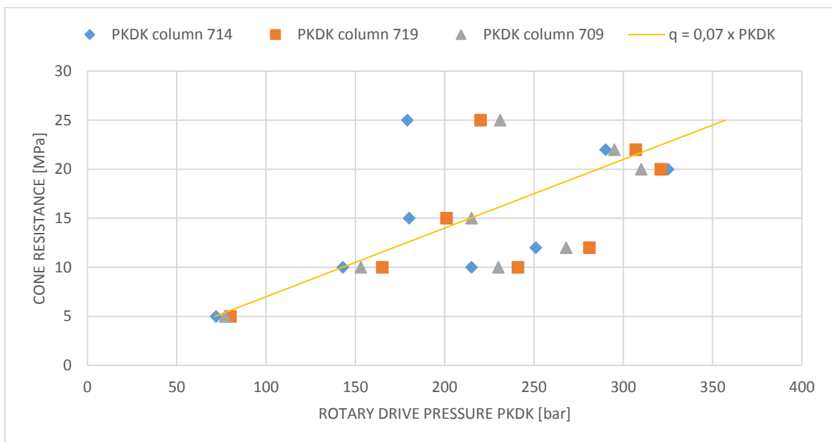
Figure S 2. PKDK dependence on q_c on the last 2 m section of the 709, 714, and 719 column cavities in cohesive soils along.
