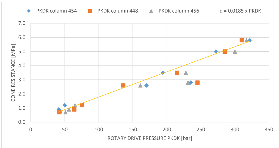
Figure S 1. PKDK dependence on q_c on the last 2 m section of the 454, 448, and 456 column cavities in cohesive soils along.
