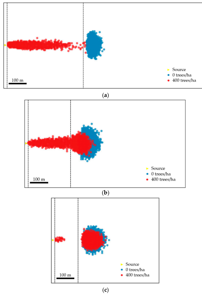
Figure 7. Maps of deposited blocks in the case of a spherical block with a unitary volume. Upper and lower limits of the transit zone (zone 2) are indicated in black dashed lines. The blue area refers to the scenario with 0 trees/ha, while the red one refers to the scenario with 400 trees/ha. Slope inclination \omega_2 : (a) 30^\circ , (b) 45^\circ and (c) 60^\circ .
