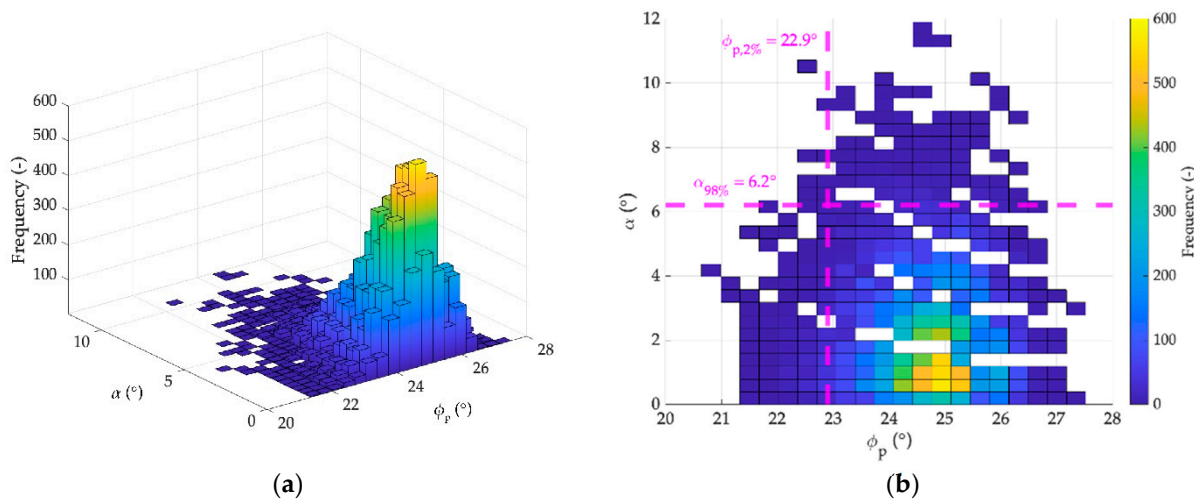
Figure 5. Example of the frequency distribution obtained for the set of 20,000 launches described in Figure 4: (a) three-dimensional histogram; (b) two-dimensional view of the same histogram. The magenta vertical and horizontal lines highlight the value of \phi_{p,2\%} and \alpha_{98\%} , respectively.
