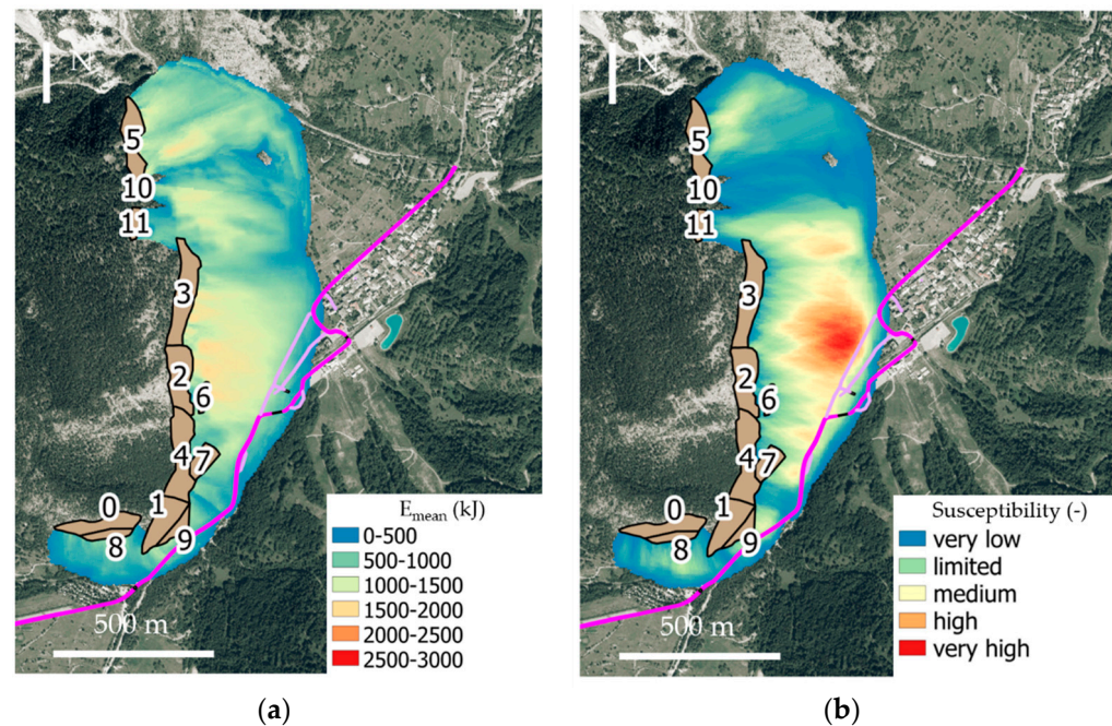
Figure 18. QPROTO results for the site of Melezet. Source areas are shown in light brown, local viability in pink, provincial road no. 216 in magenta, bridges in black. (a) Mean energy in kJ, (b) susceptibility. Orthophoto AGEA 2018.
