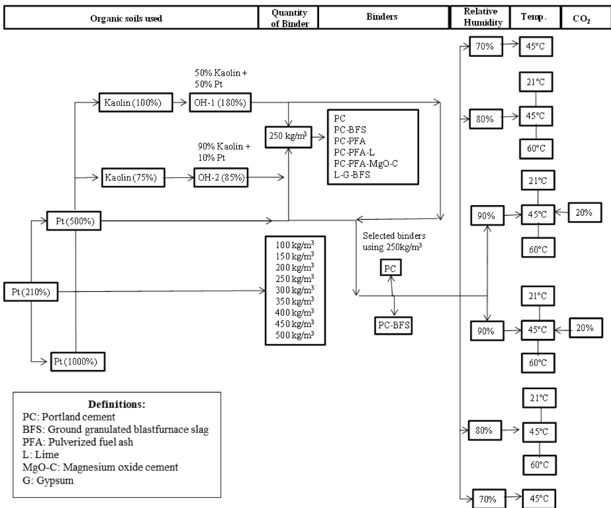
Figure 1. Flow diagram of the experimental design.
