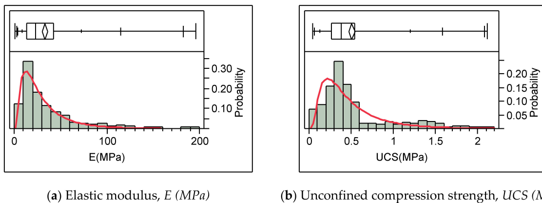
Figure 9. Relative frequency histograms and lognormal fits of response variables (a) Elastic Modulus ( E ), and (b) Unconfined Compression Strength ( UCS ).
