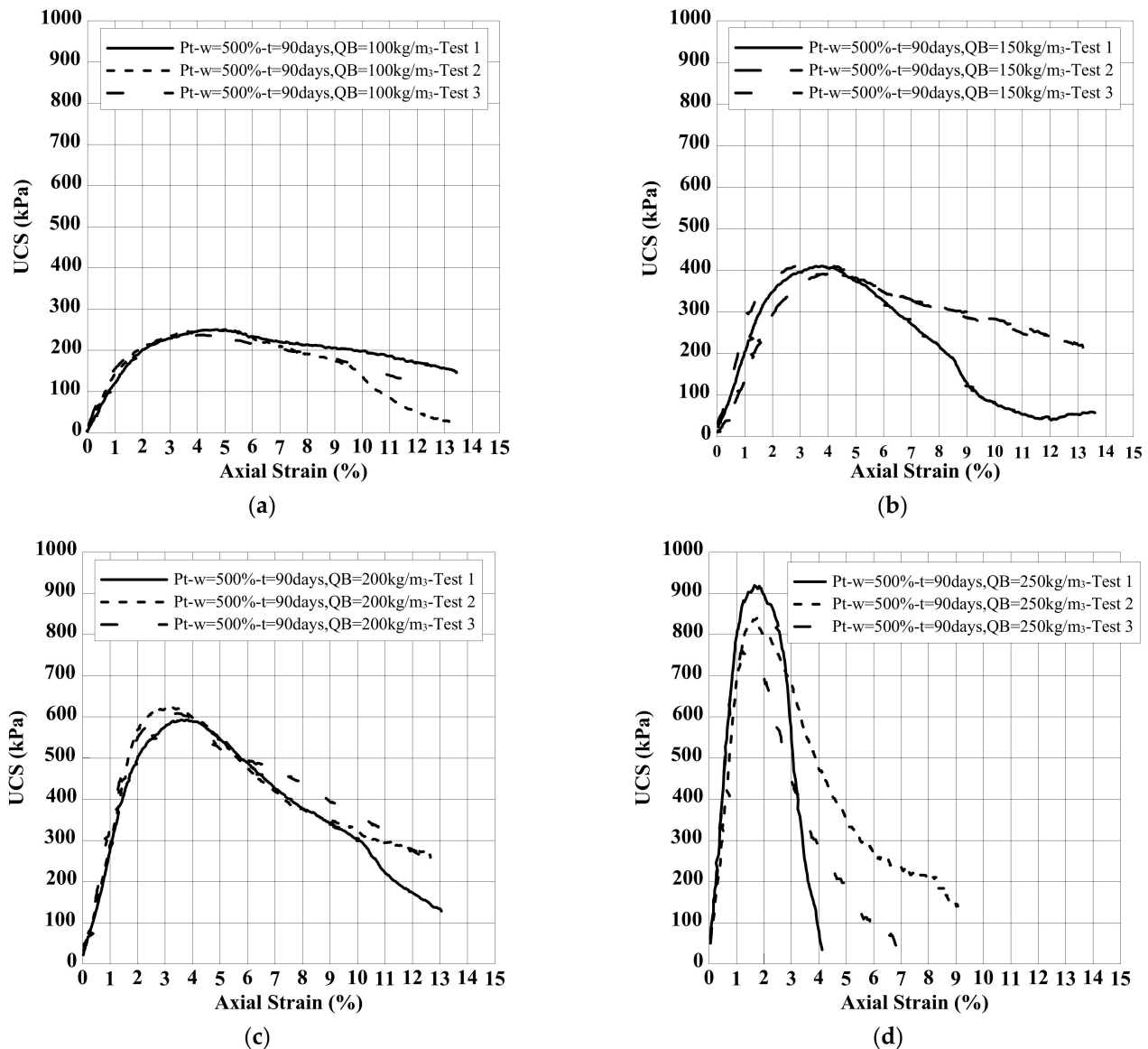
Figure 5. Axial stress–strain curves showing testing repeatability for Pt-PC-w = 500\%-t = 90 days; (a) QB = 100 \text{ kg/m}^3 ; (b) QB = 150 \text{ kg/m}^3 ; (c) QB = 200 \text{ kg/m}^3 ; and (d) QB = 250 \text{ kg/m}^3 .
