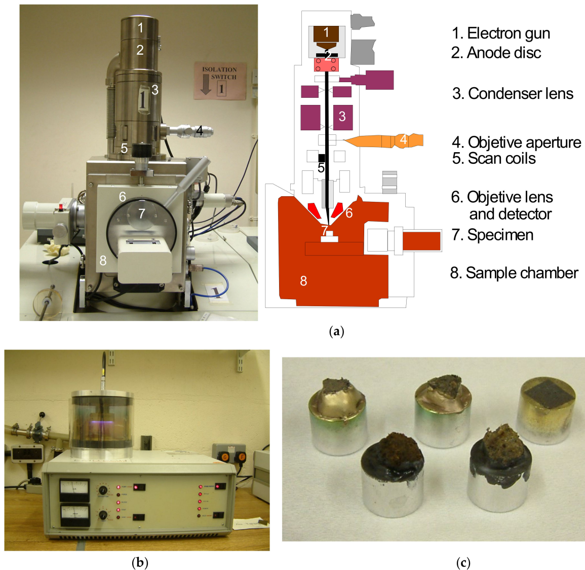
Figure 6. SEM and vacuum coating equipment: (a) SEM's main components, (b) coating of samples with gold and (c) samples before and after coating.
