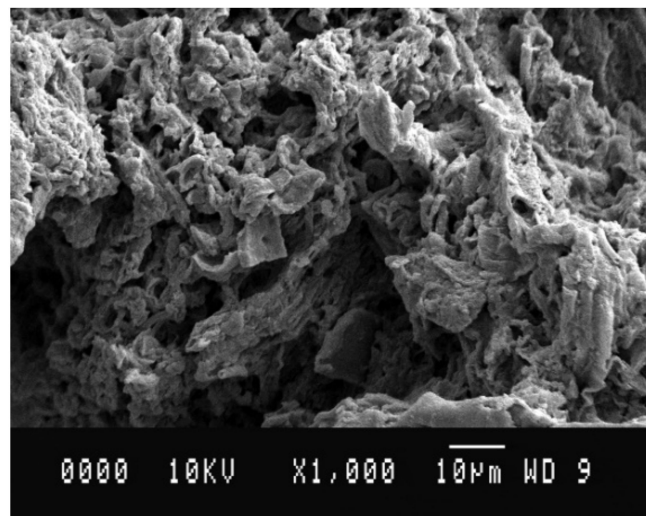
Figure 15. Typical SEM microimages of the Pt studied at a magnification of 1000.
