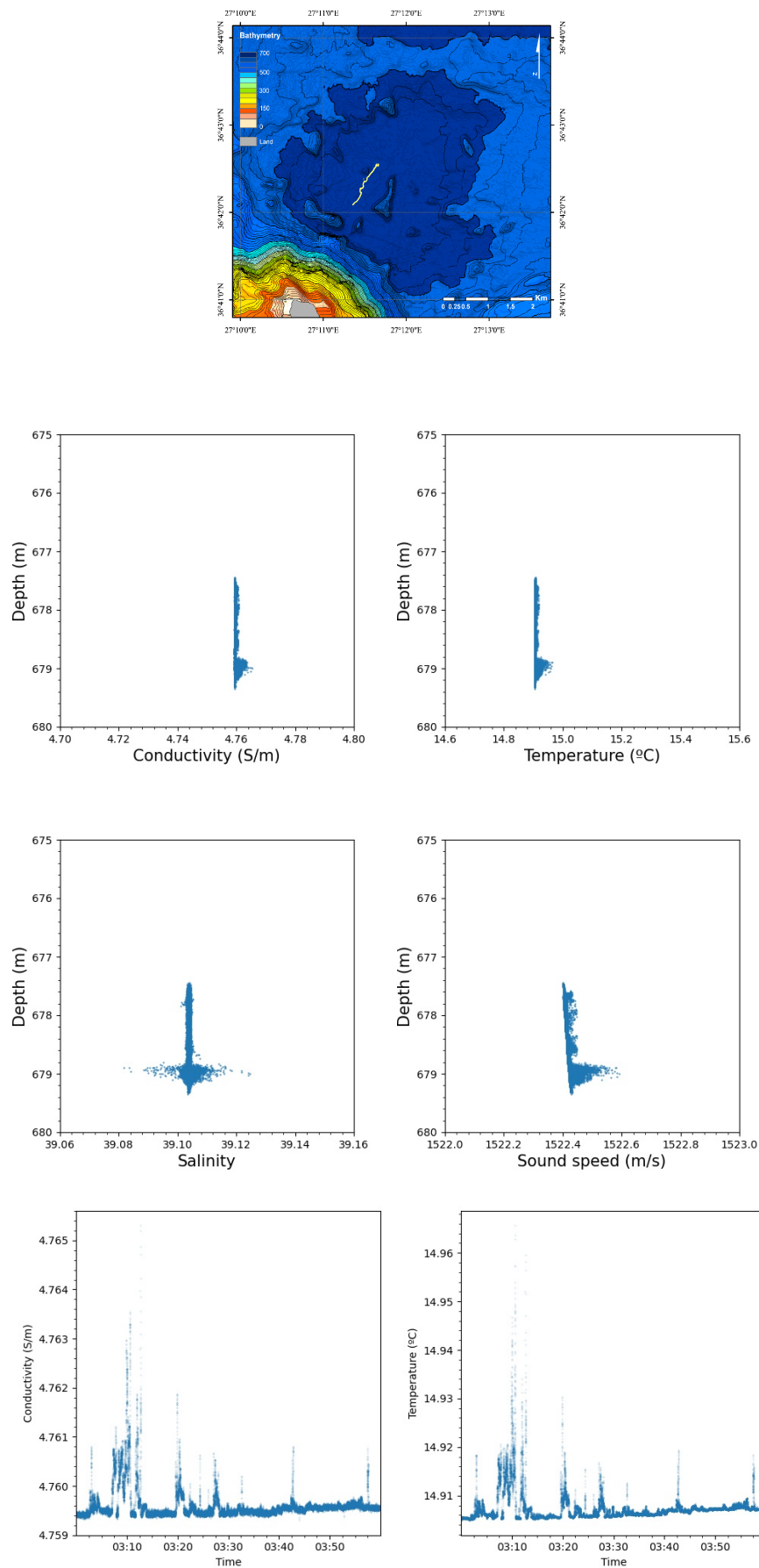
Figure A9. Track 9 (top row), Vertical Profiles (middle rows) and time series (bottom row).
