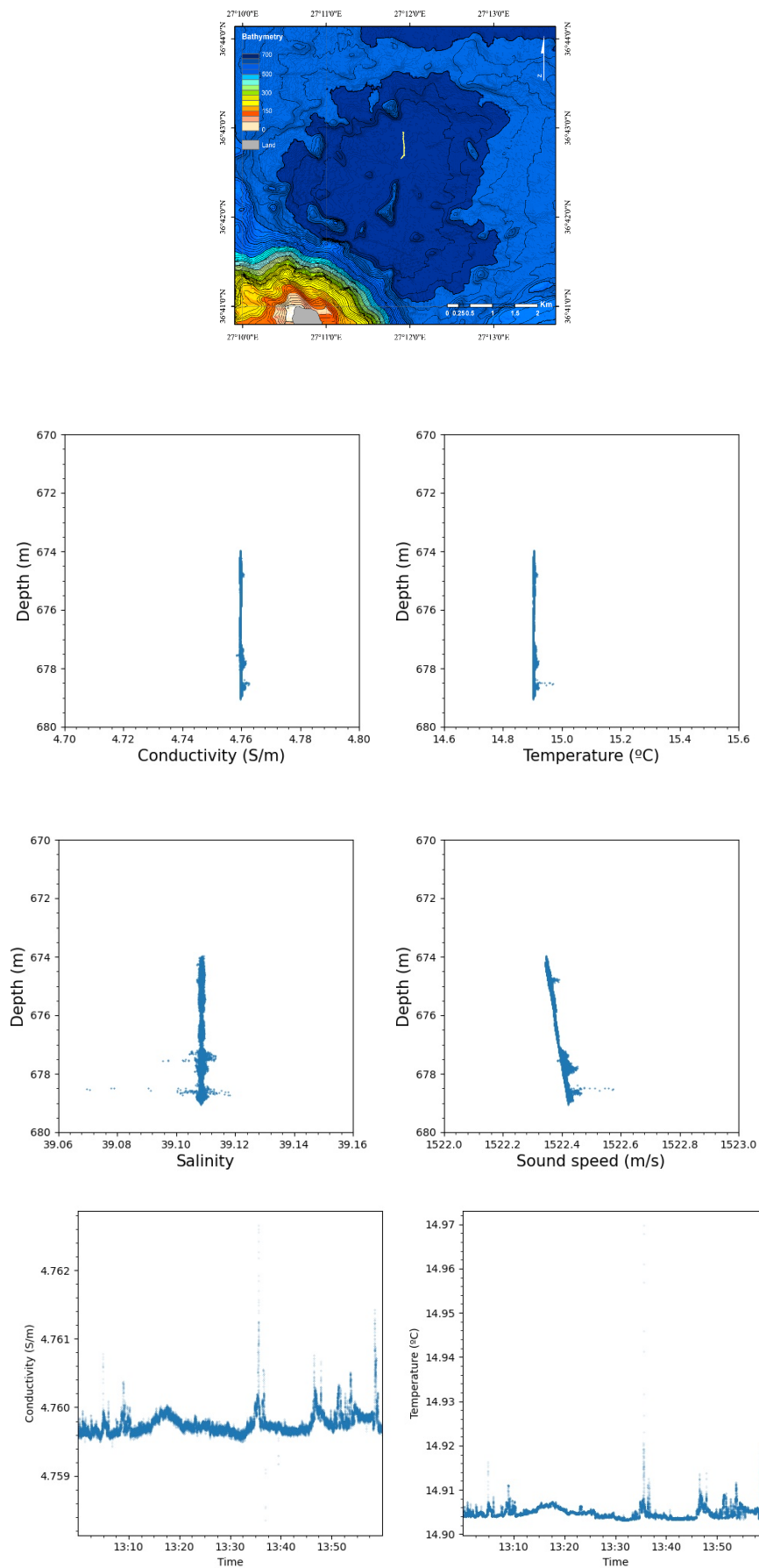
Figure A2. Track 2 (top row), Vertical Profiles (middle rows) and time series (bottom row).
