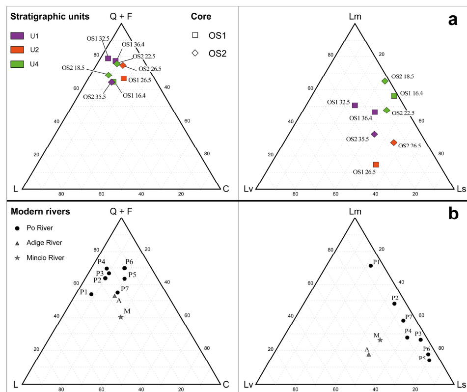
Figure 5. Composition of sands from Ostiglia cores and modern rivers. Ternary diagrams showing composition of sands from cores OS1 and OS2 (a) and from modern rivers (b). Q + F: quartz and feldspar; L: siliciclastic lithics; C: carbonate lithics; Lm: metamorphic lithic; Lv: volcanic lithic; Ls: sedimentary lithic.
