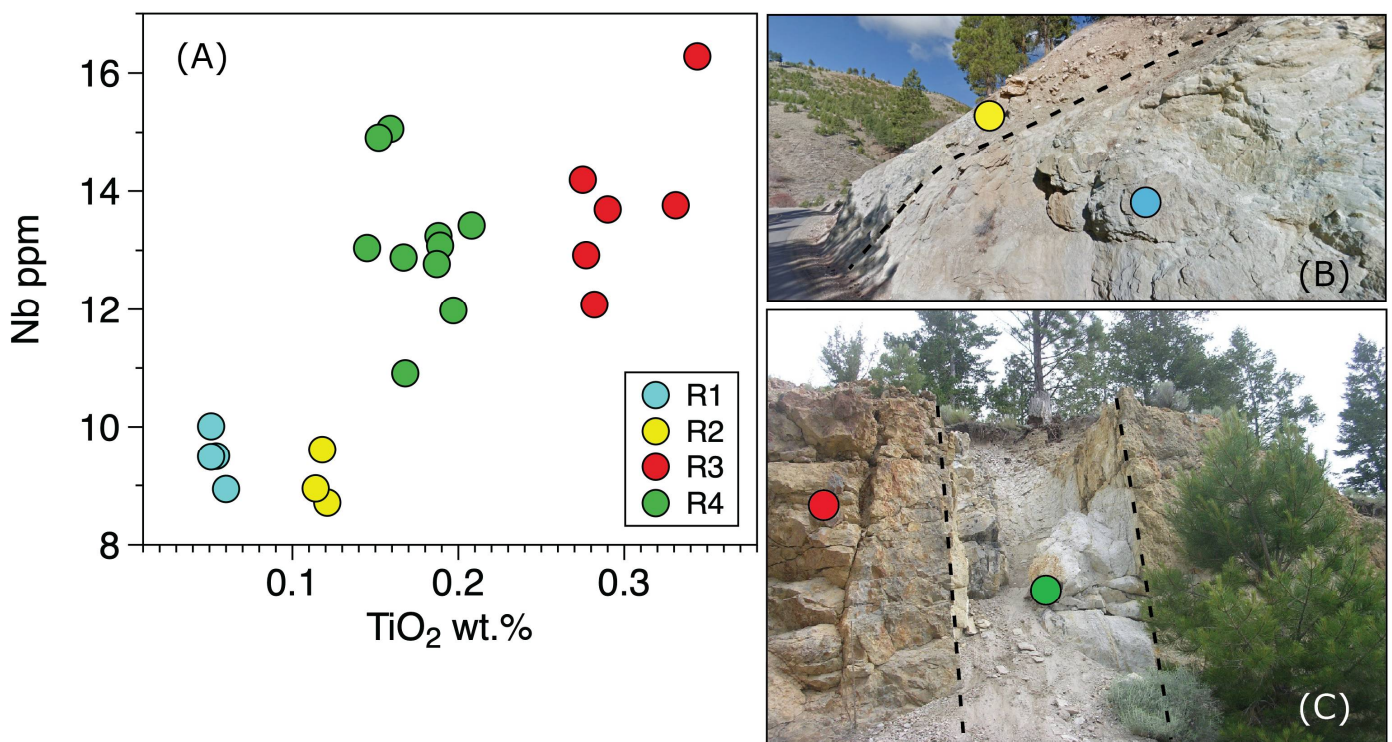
Figure 5. Field relationships and composition of Dooley Mountain rhyolites, the northernmost rhyolite center (after [54]). (A) Rhyolites are divided into 4 compositional groups, R1 through R4; (B) R2 rhyolite overlies R1 rhyolite; (C) Tuff dike with glassy matrix and vertically oriented fiammes with a R4 composition cut rhyolite breccia of a R3 rhyolite.
