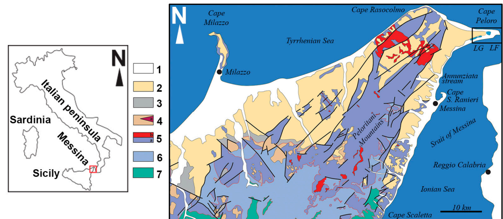
Figure 1. Geological sketch map of the NE sector of the Peloritani Mountains (NE Sicily). The black rectangle on the Cape Peloro peninsula (NE edge of Messina) evidences the sector of the coast studied (see Figure 2). In this peninsula, the Cape Peloro lagoon area (coastal lakes in sky blue color) is formed by Lake Ganzirri (LG) and Lake Faro (LF). Legend: (1) Alluvial and beach deposits (Holocene). (2) Miocene–Pleistocene sedimentary successions (including the Pleistocene Messina Fm). (3) Floresta calcarenites (Langhian–upper Burdigalian) and Antisicilide Complex (lower Miocene–upper Cretaceous). (4) Stilo–Capo d’Orlando Formation (Burdigalian) with olistoliths (a). (5) Aspromonte Unit (a: Variscan metamorphic basement; b: Plutonic basement). (6) Mela Unit (Variscan metamorphic basement). (7) Mandanici–Piraino Unit (Variscan metamorphic basement and Mesozoic cover). The red square on the insert on the left represents the extension of the geological sketch map. The map was modified after [27].
