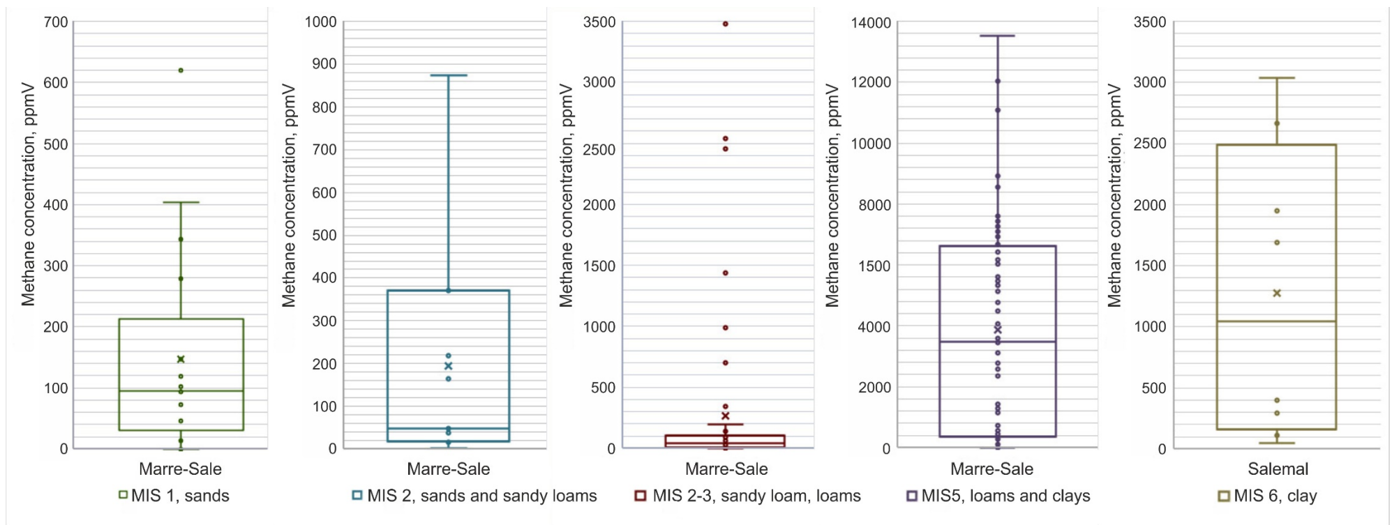
Supplementary Figure 1. Methane concentration in typical permafrost sediments of the study region (presented as box-plots).
