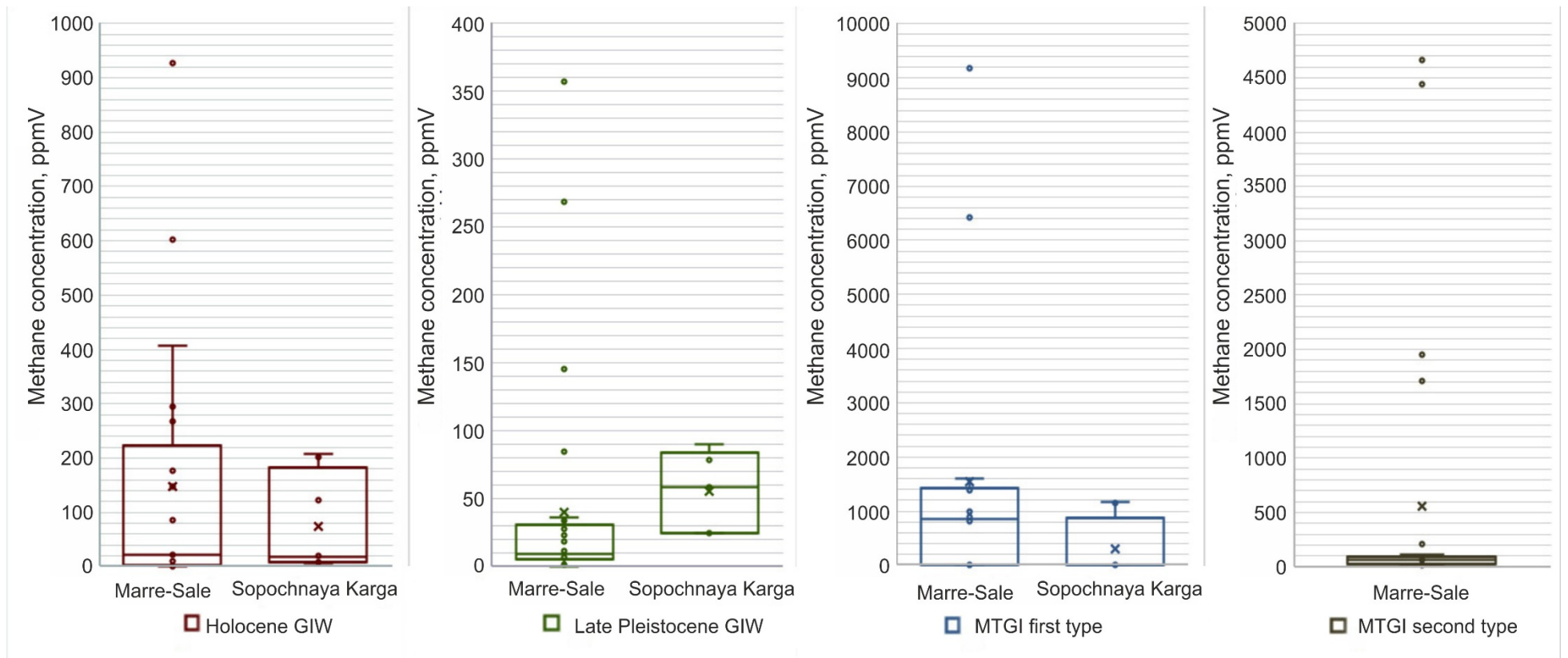
Supplementary Figure 2. Methane concentration in air bubbles of ground ice wedges (GIW) and massive tabular ground ice (MTGI) of Marre-Sale and Sopochnaya Karga (presented as box-plots).
