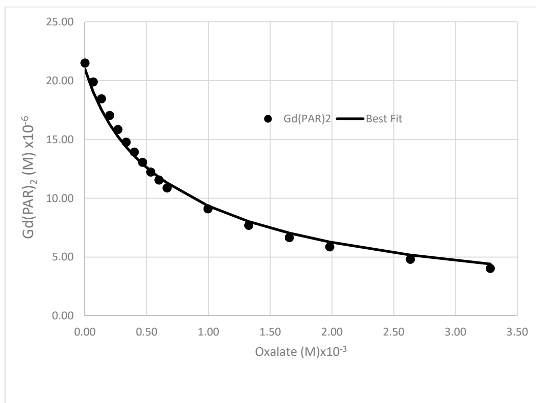
Figure 4. The reduction of Gd(PAR)_2 concentration with increasing oxalate concentration at pH 8 at 25 °C is presented. The experimental data have been fit to Equation (4).
