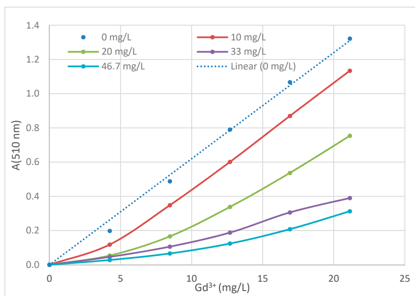
Figure 8. The data for the titration with Gd 3+ of Pahokee Peat humic acid at pH 8 and at various concentrations is summarized in this figure. The curvature in the plot indicates finite complexing capacity.
