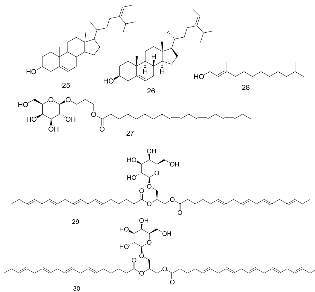
Figure 8. Compounds from 25–28 (phyosterols, glycolipid, and farnesol) and compounds 29 and 30 (Diacylglyceroglycolipids).
