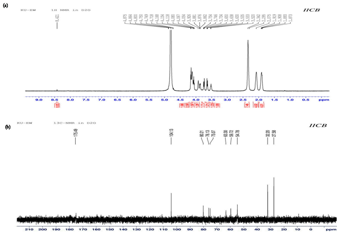
Figure 1. (a) 1 H Nuclear Magnetic Resonance (NMR) and (b) 13 C NMR signal positions of extracellular polymeric substance (EPS).
