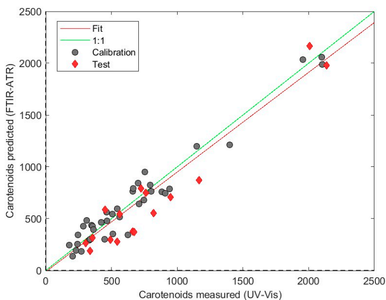
Figure 3. Regression line of the PLS model for total carotenoid content (in \mu\text{g/g} , dry basis) obtained from freeze-dried samples. In grey circles ( \bullet ), the training set; in red rhombuses ( \blacklozenge ), the prediction set.
