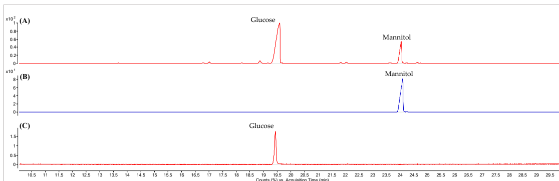
Figure 5. GC-MS chromatograms of acetylated methyl glycosides from RSLDE OUT (A); acetylated mannitol (B); acetylated methyl glycoside of glucose (C).
