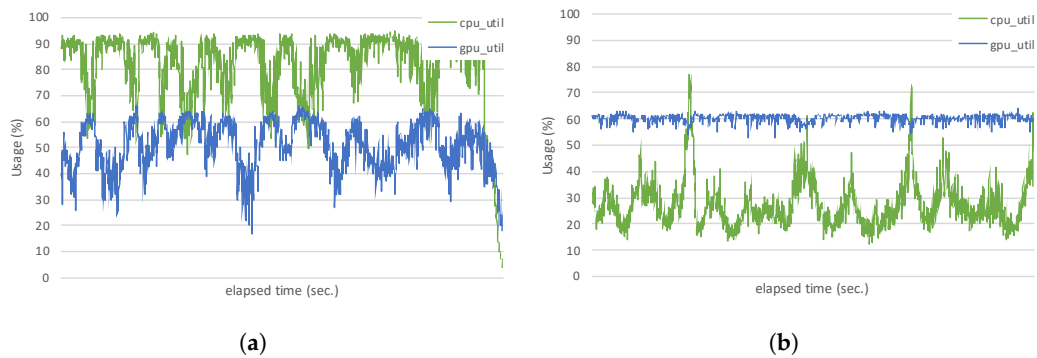
Figure 5. Comparison of CPU and GPU usages (%) of ASR systems using the baseline acoustic score computation method for (a) LSTM-based AM and (b) BLSTM AM with the test set. The green and blue lines indicate the CPU and GPU usages.
