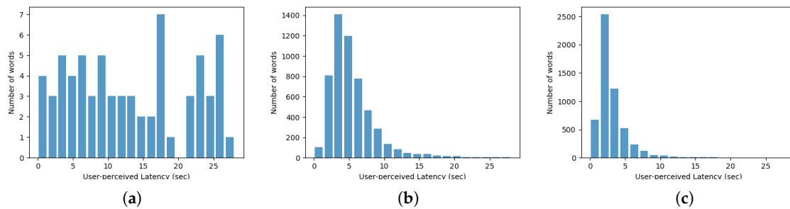
Figure 8. Histogram of the user-perceived latency for all words in test set 1. (a) Without VAD (b) With VAD, minibatch 200 (c) With VAD, minibatch 100.
