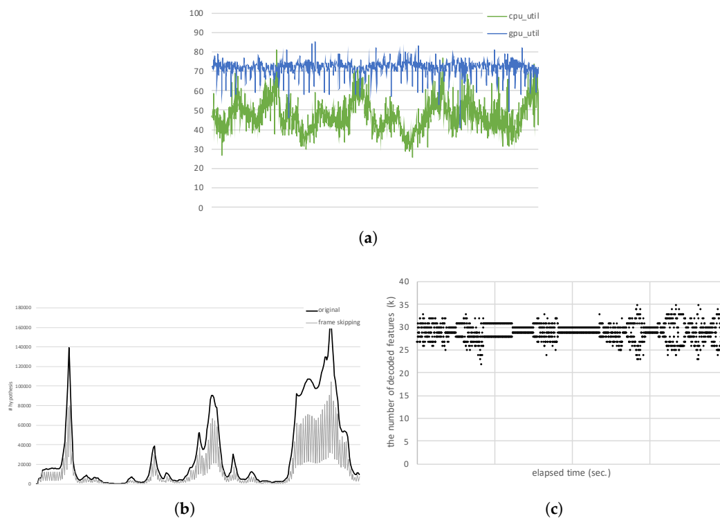
Figure 7. Performances of an ASR system using both the proposed fast parallel acoustic score computation method of BLSTM AM and the frame skip method, with the test set, in terms of (a) CPU and GPU usages (%), (b) number of hypothesis during Viterbi decoding, and (c) the number ( k ) of parallel decoded feature vectors of the proposed method for each acoustic score computation time. The green and blue lines indicate the CPU and GPU usages, and the straight and dotted lines indicate the proposed decoding without/with frame skip.
