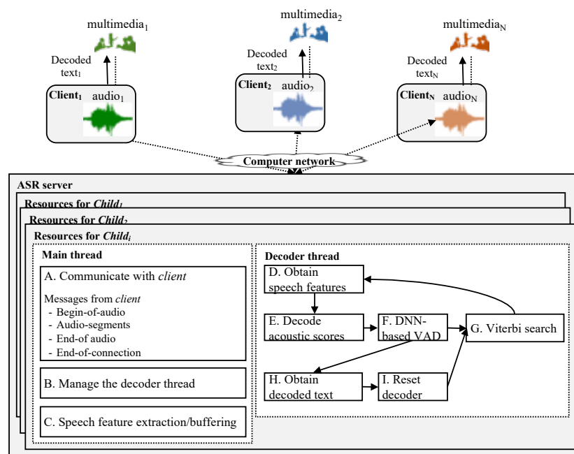
Figure 1. Overall structure of the server-client-based online automatic speech recognition (ASR) system used in this paper.
