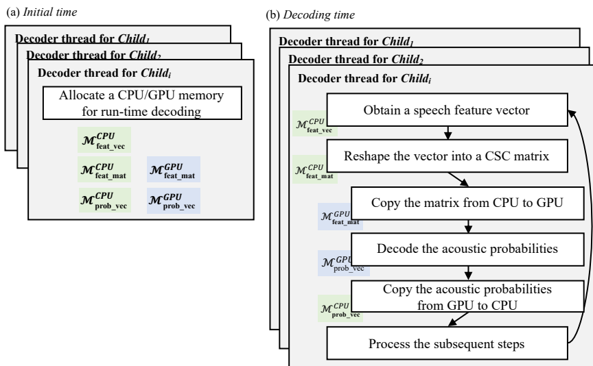
Figure 3. Main procedure of the baseline multichannel acoustic score computation based on CSC bidirectional long short-term memory acoustic model (BLSTM AM). The green- and blue-shaded boxes indicate the CPU and GPU memories, respectively.
