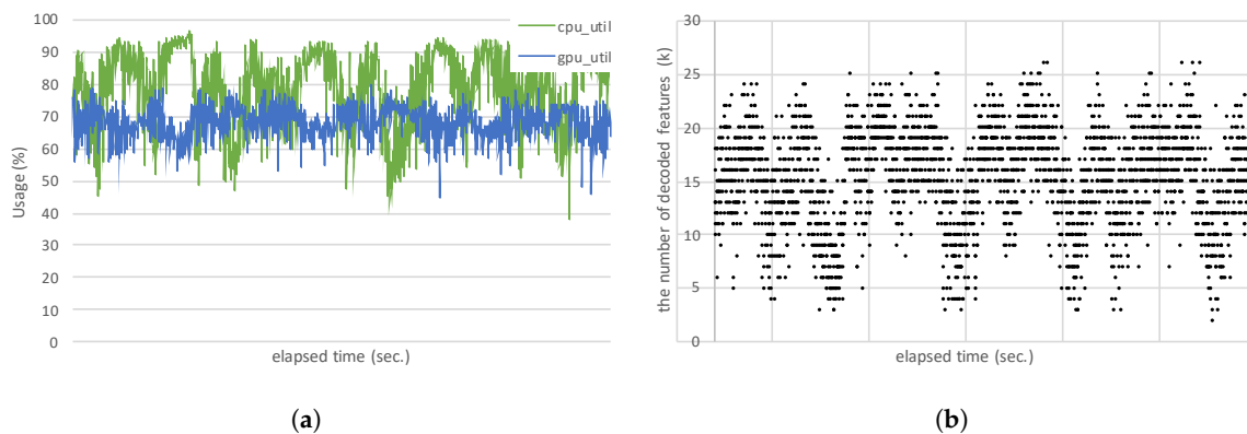
Figure 6. Performances of an ASR system using the proposed fast parallel acoustic score computation method of BLSTM AM with the test set, in terms of (a) CPU and GPU usages (%) and (b) the number ( k ) of parallel decoded feature vectors of the proposed method for each acoustic score computation time. The green and blue lines indicate the CPU and GPU usages, respectively.
