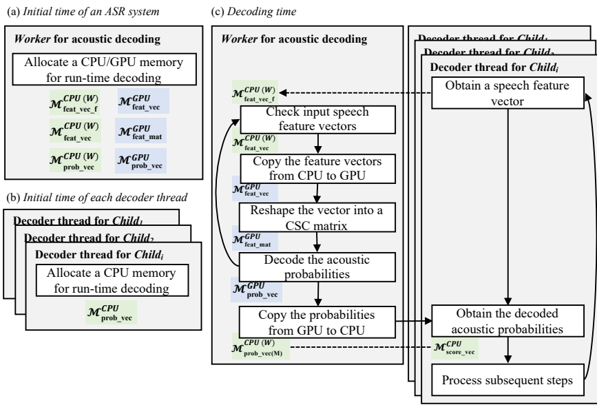
Figure 4. Main procedure of the proposed fast multichannel parallel acoustic score computation using a CSC BLSTM AM. The green- and blue-shaded boxes indicate a CPU memory and a GPU memory, respectively.
