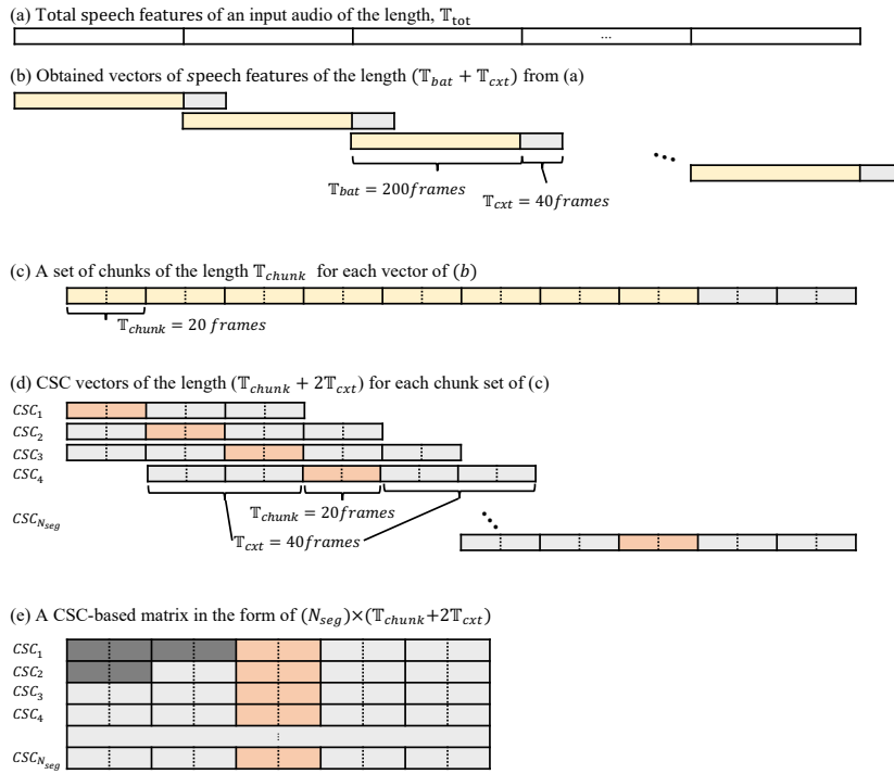
Figure 2. Context-sensitive-chunk (CSCs) of our ASR system with T_{bat} of 200 frames, T_{chunk} of 20 frames, and T_{cxt} of 40 frames: (a) extracted speech features from the overall input sequence, (b) a set of speech feature vectors where each vector is obtained from \mathcal{R}_{feat} and the size is (T_{bat} + T_{cxt}) , (c) a set of chunks where the chunk size is T_{chunk} , (d) a set of CSCs where the CSC size is (T_{cxt} + T_{chunk} + T_{cxt}) , and (e) a CSC matrix for a speech feature vector.
