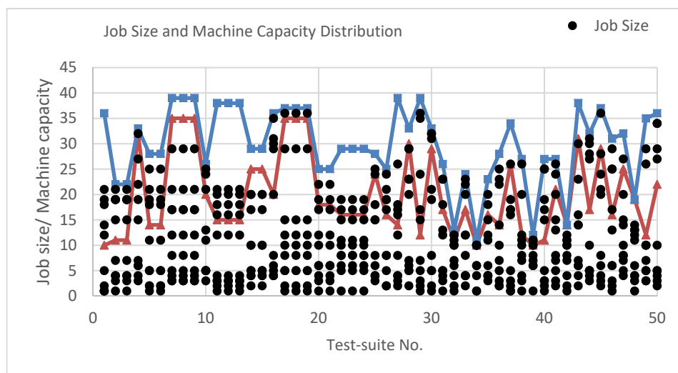
Figure 2. Job size and machine capacity distribution.
