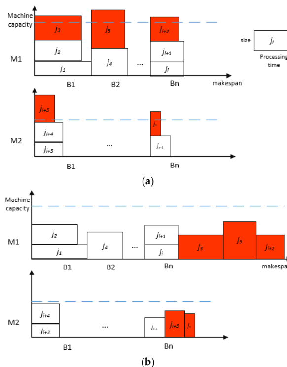
Figure 1. Illustration of the 4.5-approximation algorithm. (a) The 4.5-approximation algorithm with one-job-overfull batches. (b) The 4.5-approximation algorithm with a feasible schedule.
