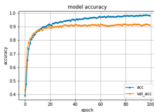
Figure 11. The accuracy of 3DCNN model during training.
