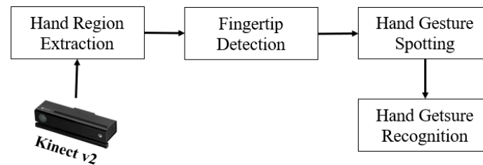
Figure 1. Algorithm pipeline.
