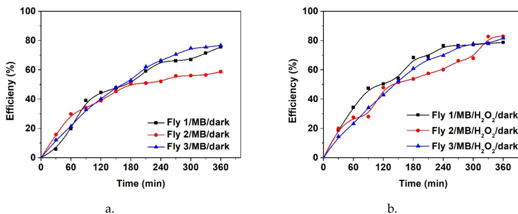
Figure S2. The adsorption process on Fly ash-TiO 2 materials: (a) without H 2 O 2 and (b) with H 2 O 2 .
