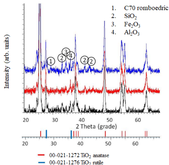
Figure S1. The XRD pattern of Fly ash-TiO 2 materials: Fly1 (black), Fly2 (red) and Fly 3 (blue).
