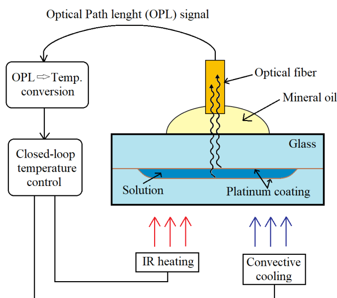
Figure 9. Schematic representation of interferometric temperature control system. Adapted from [48]. Copyright 2012 © The Royal Society of Chemistry.
