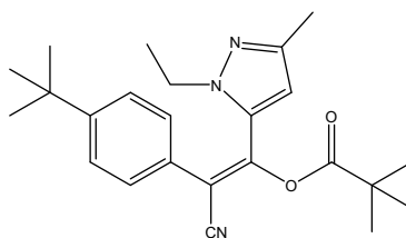
Figure S1. Structure of SYP-9625.
