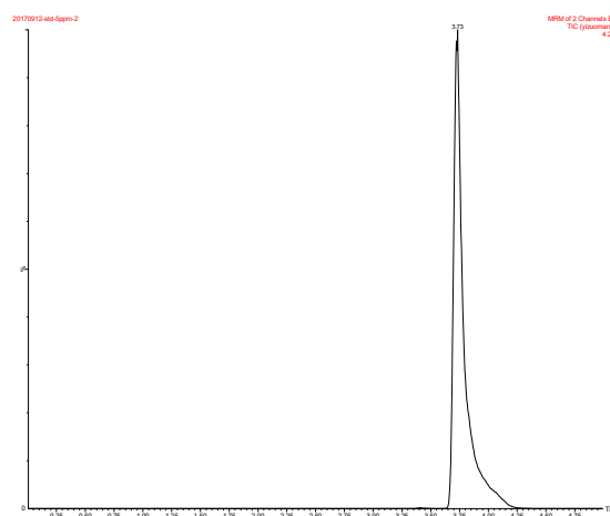
Figure S2. The UPLC-MS chromatogram for SYP-9625.
