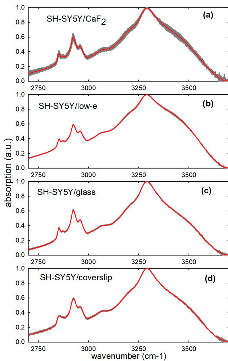
Figure.2 SI. Distribution of the measured FTIR spectra of SH-SY5Y cells grown on CaF 2 crystals (a), low-e slide (b), glass slide (c) and glass coverslip (d). The shaded area corresponds to average spectrum ± standard deviation values.
