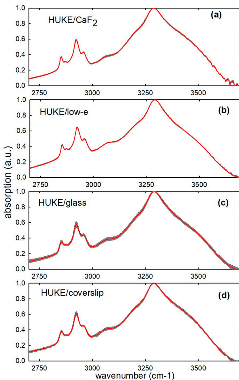
Figure S1. Distribution of the measured FTIR spectra of HUKE cells grown on CaF 2 crystals (a), low-e slide (b), glass slide (c) and glass coverslip (d). The shaded area corresponds to average spectrum ± standard deviation values.
