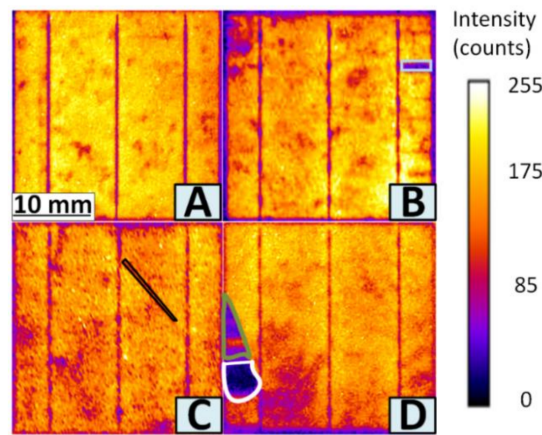
Figure 1. EL cell images inflicted with different faults: (A) no failures; (B) finger failures (region marked with light blue); (C) micro-crack Mode A (black); (D) cracks Mode B (olive green) and Mode C (white).
