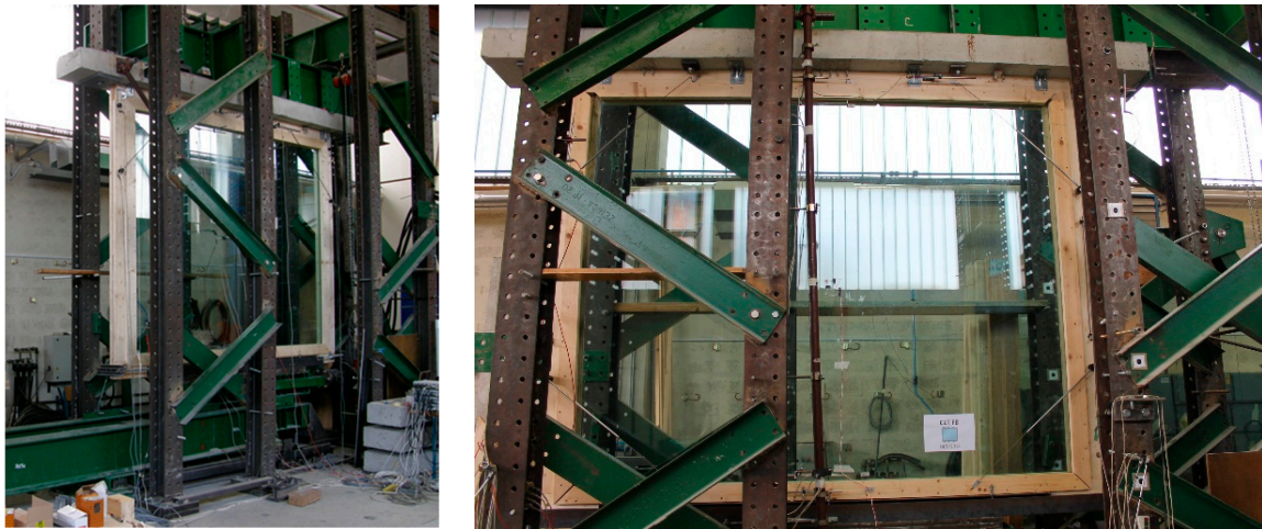
Figure 4. An example of a timber–glass composite system [39,40,88–94].
