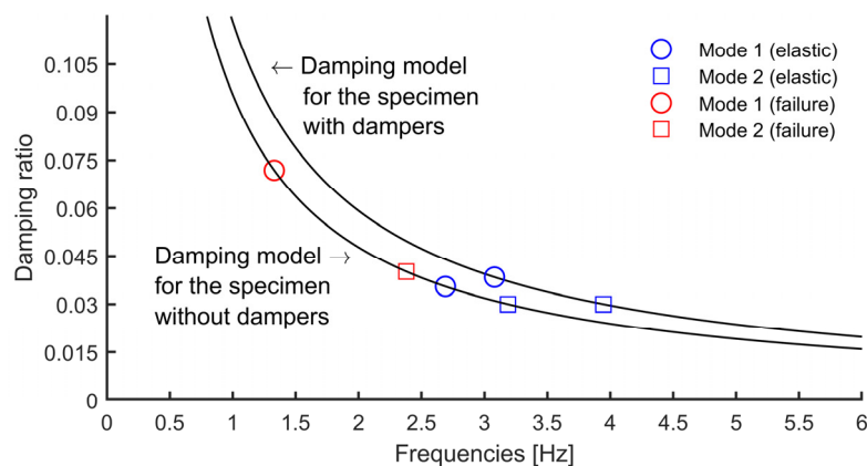
Figure 9. Mass-damping model defined for waffle-flat-plate (WFP) system with and without dampers.
