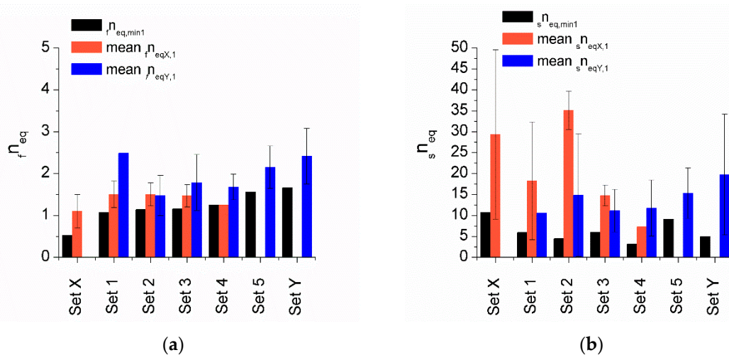
Figure 15. Equivalent number of cycles obtained in the analyses at the first story for WFP system (a) and for hysteretic dampers (b).
