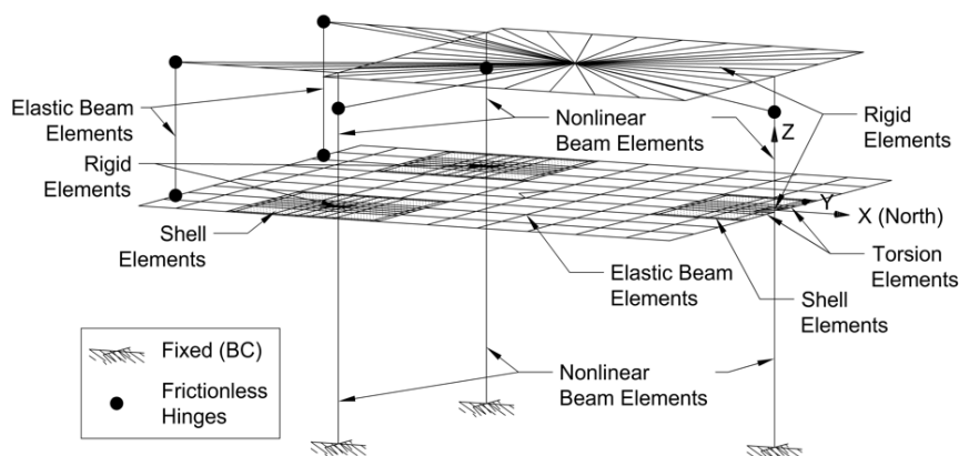
Figure 3. Overview of the numerical model.
