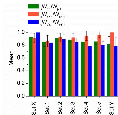
Figure 13. Ratio of the dissipated energy in the hysteretic dampers with respect to the total value at the first story, overall ( {}_sW_{p,1}/W_{p,1} ), and by components ( {}_sW_{pX,1}/W_{pX,1} and {}_sW_{pY,1}/W_{pY,1} ).
