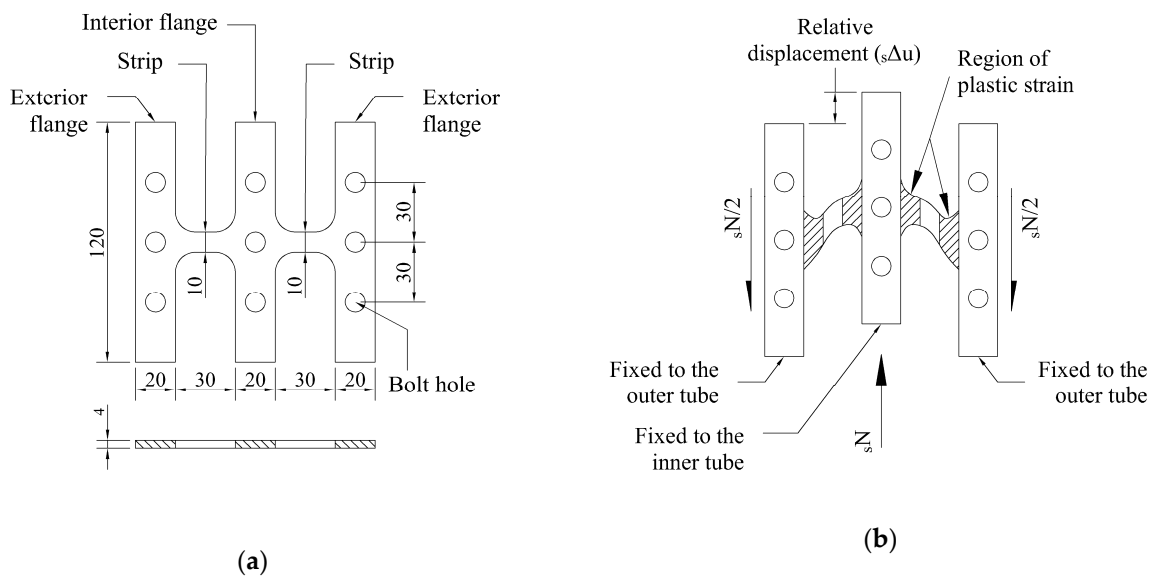
Figure 6. Slit-plate dampers: (a) dimensions (in mm); (b) deformed shape.
