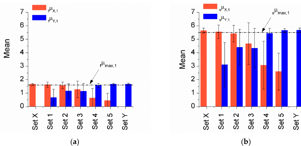
Figure 12. Mean and error bars for f\mu along X and Y directions: (a) main structure; (b) hysteretic dampers.
