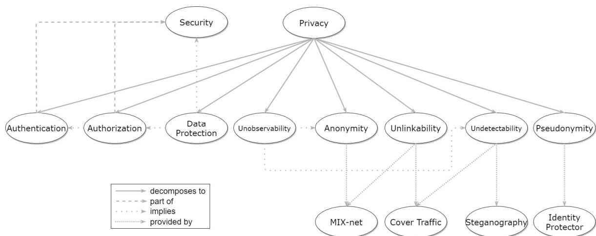
Figure 19. Hierarchical graph of Privacy properties and relevant patterns.
