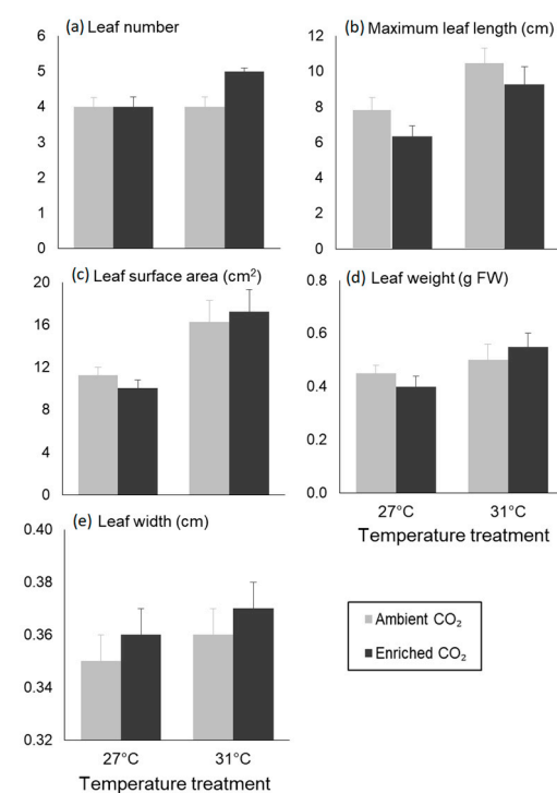
Figure 2. The effect of increasing temperature and CO 2 enrichment on (a) leaf number, (b) maximum leaf length, (c) leaf surface area, (d) leaf weight, and (e) leaf width of Enhalus acoroides seedlings at the end of the experimental period. Values are mean \pm SE (n = 6).
