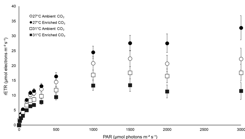
Figure 4. Rapid light curves. Relative electron transport rates ( rETR ) of 13 measurements at increasing photosynthetic active radiation (PAR) measured on leaves of seedlings under the four experimental treatments at the end of the experimental period. Values are mean \pm SE ( n = 6 ).
