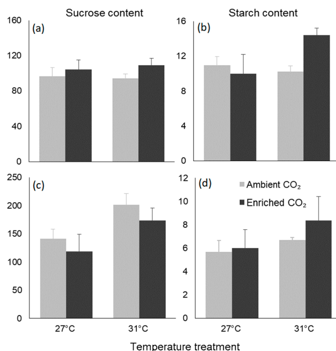
Figure 6. The effect of increasing temperature and CO 2 enrichment on sucrose (left column) and starch (right column) content (sucrose equivalents g -1 DW) on leaves (a,b) and seeds (c,d) in seedlings of Enhalus acoroides at the end of the experimental period. Values are mean ± SE (n = 3 for leaves and n = 6 for seeds).
