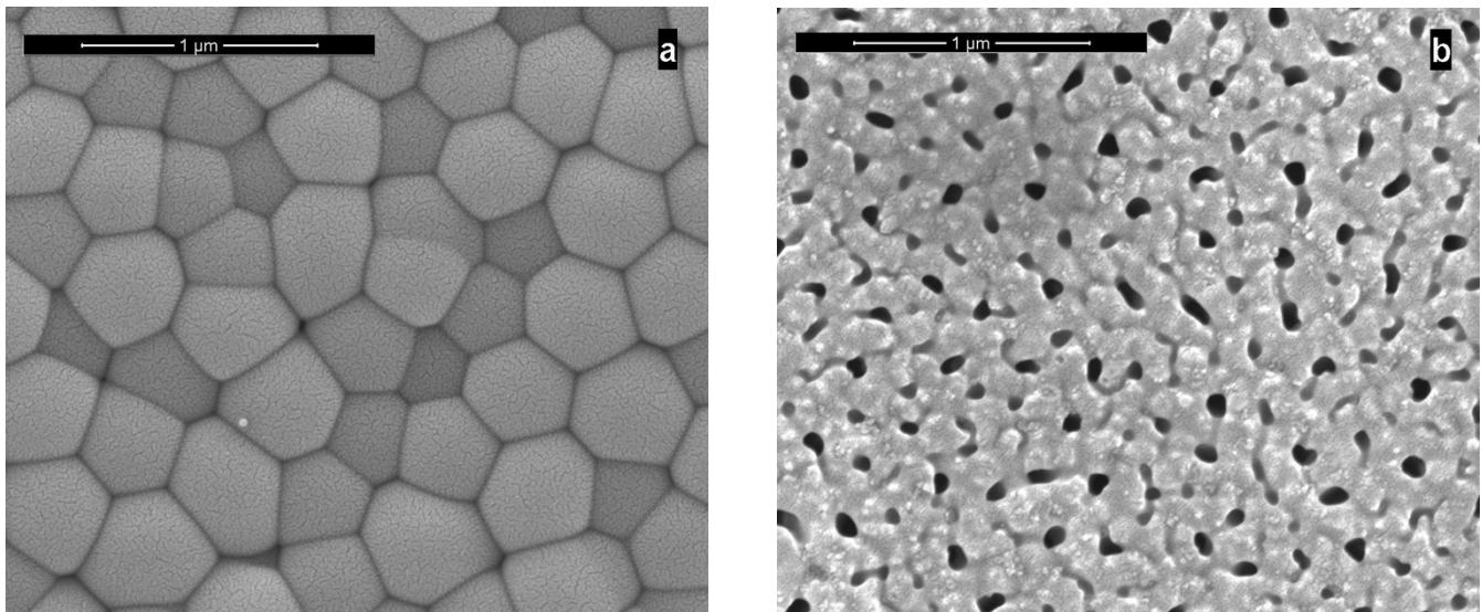
Figure 4. FESEM images of PAA formed at 160 V and 0 °C in 0.4 M H 3 PO 4 and 0.095 M Al(OH) 3 after passing 20 C cm -2 : (a) inner and (b) outer surface.
