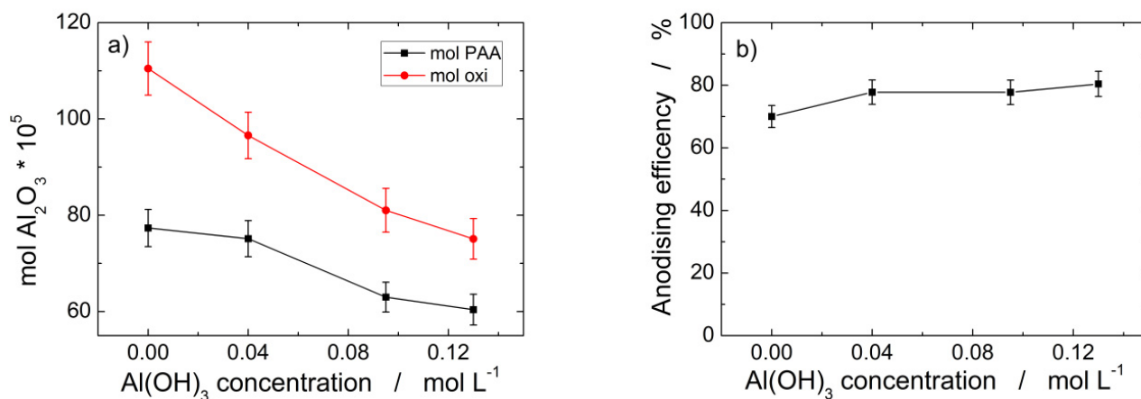
Figure 2. Aluminum anodization in mixed 0.4 M H 3 PO 4 /Al(OH) 3 electrolytes at 160 V and 0 °C after 160 C cm -2 vs. Al(OH) 3 concentration: (a) mol cm -2 of Al oxidized as Al 2 O 3 and PAA moles cm -2 formed; (b) anodizing % efficiency.
