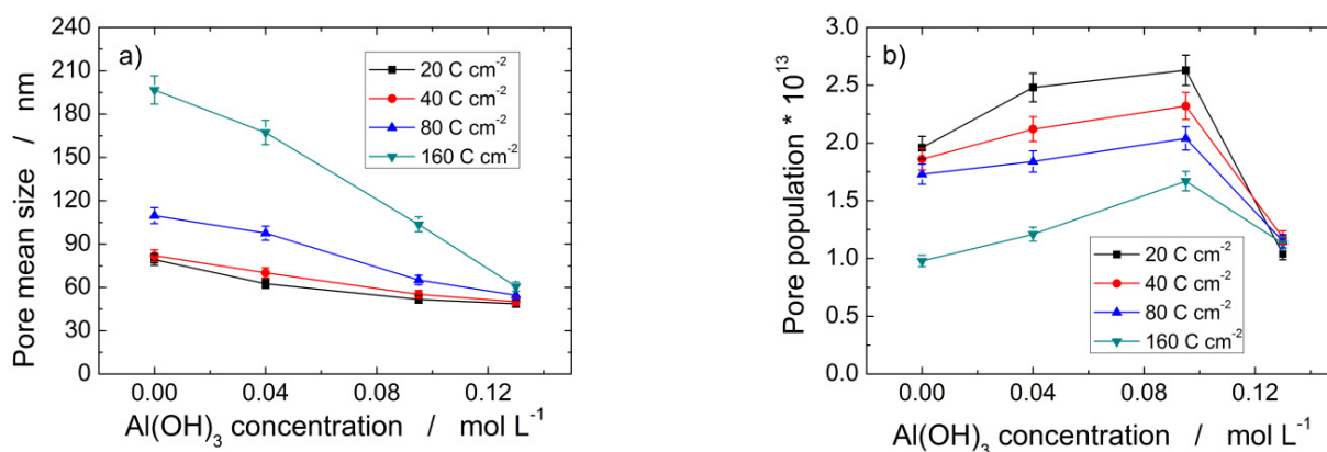
Figure 5. Pore mean size (a), and surface pore population (b) of PAA layers obtained by Al anodization at 160 V and 0 °C in 0.4 M H 3 PO 4 added with different amounts of Al(OH) 3 .
