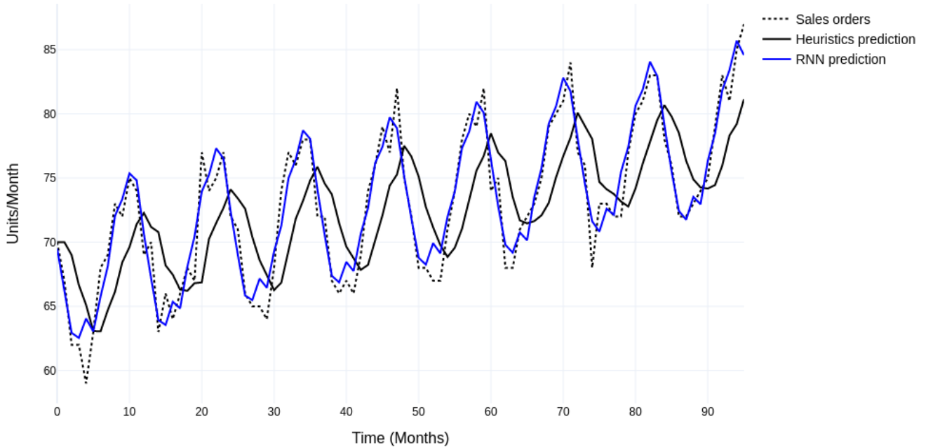
Figure 7. Comparing heuristic and RNN sales predictions.
