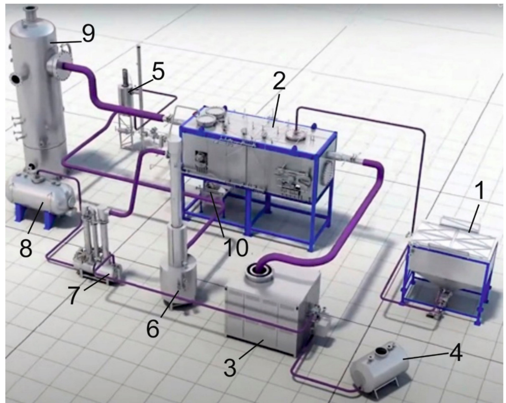
Figure 2. Setup for steam pyrolysis of OS: 1—loading unit, 2—reactor, 3—steam boiler, 4—fuel storage tank, 5—emergency combustion system, 6—stage I of steam–gas product condensation, 7—stage II of steam–gas product condensation, 8—accumulator of condensed products (water), 9—scrubber, 10—discharging loader for solid-phase products.
