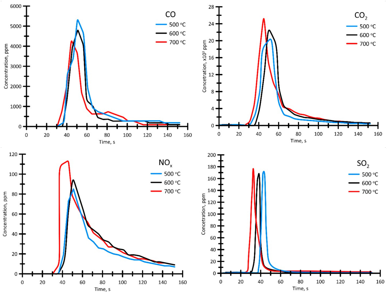
Figure 14. Concentration profiles of the release of gas-phase compounds CO, CO 2 , NO x , and SO 2 formed in the combustion of liquid hydrocarbon droplets at T_g = 500\text{--}700\text{ }^{\circ}\text{C} .
