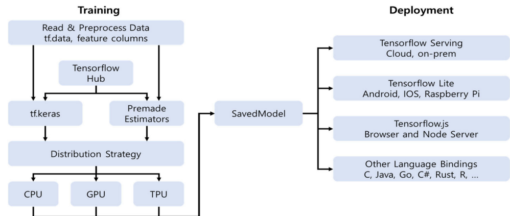
Figure 4. TensorFlow 2.0 version architecture and processing process.
