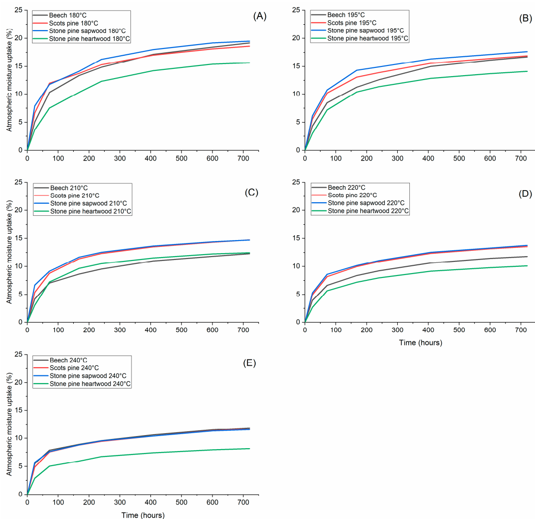
Figure 4. Relationship between maximum heat treatment temperatures and water absorption from ambient air for samples placed above water in a glass chamber (RH = 98\% \pm 2\% ): 180^\circ\text{C} (A), 195^\circ\text{C} (B), 210^\circ\text{C} (C), 220^\circ\text{C} (D), 240^\circ\text{C} (E).
